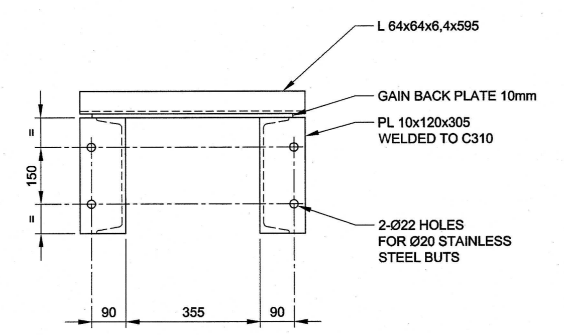
SECTION B-B 1:10
