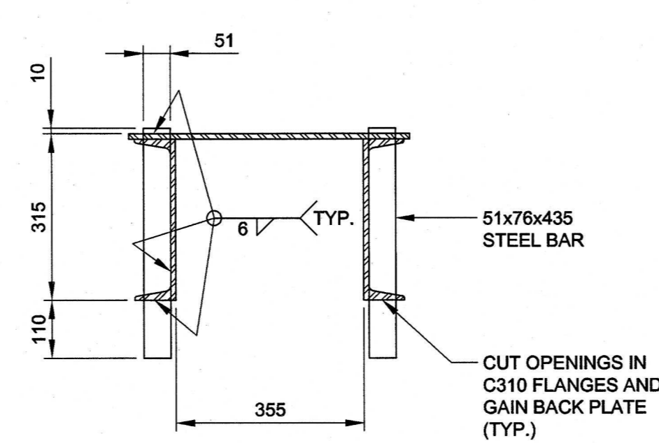
SECTION C-C 1:10 (JACKING BRACKETS DETAIL)
