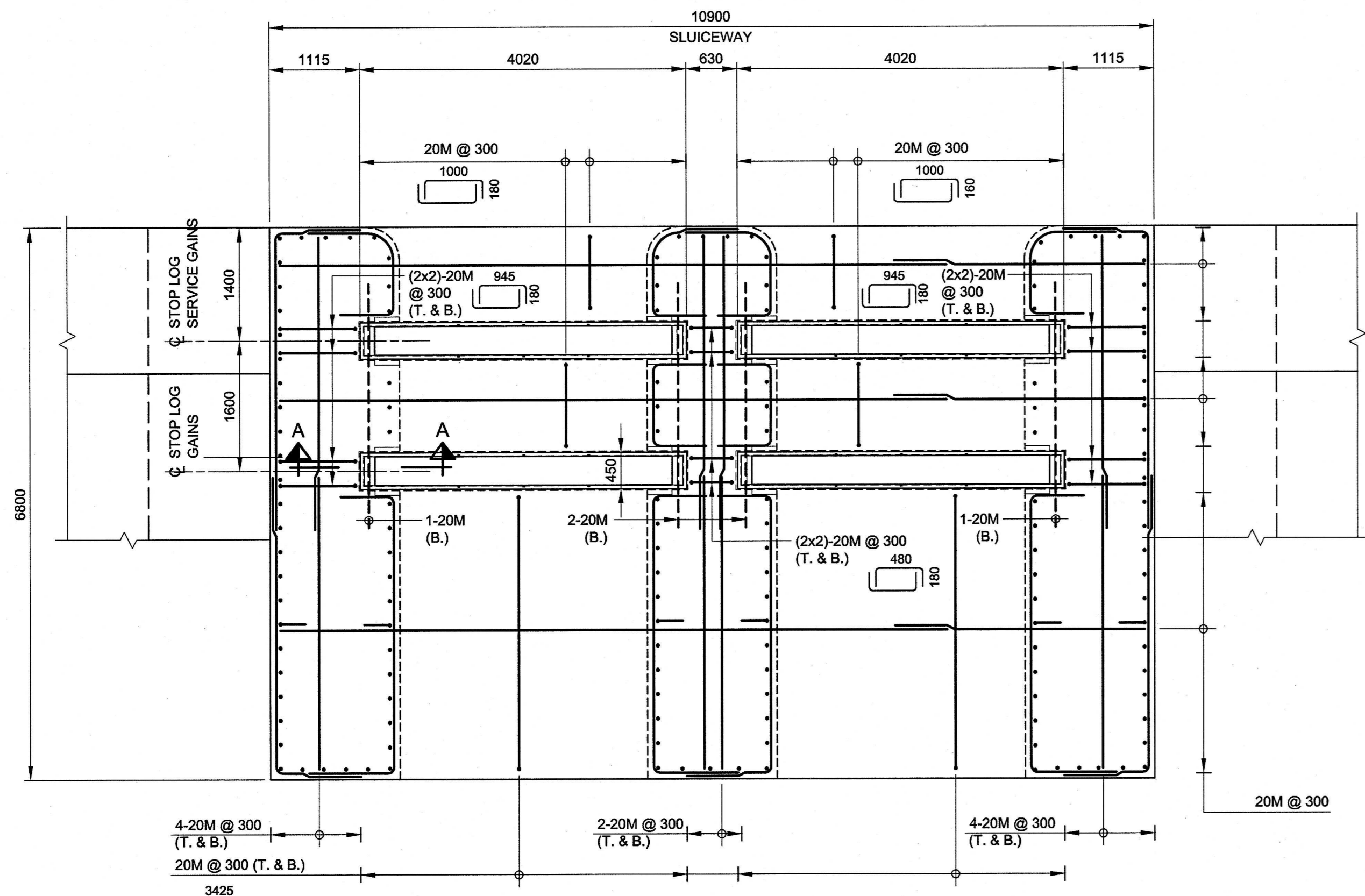
DOWNSTREAM PLAN EL. 163.500 1:50 REINFORCEMENT
