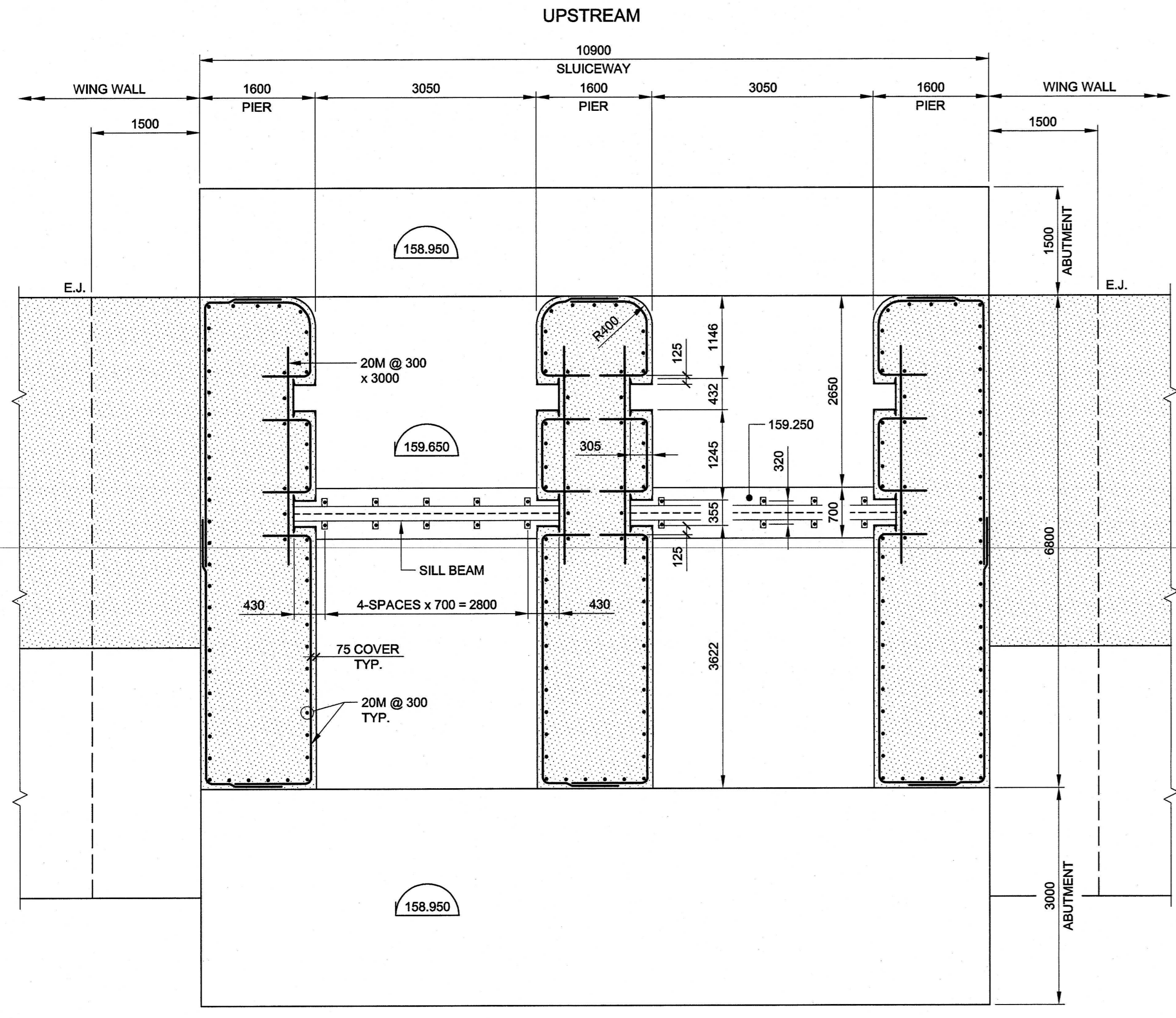
DOWNSTREAM PLAN EL. 159.650 1:50
