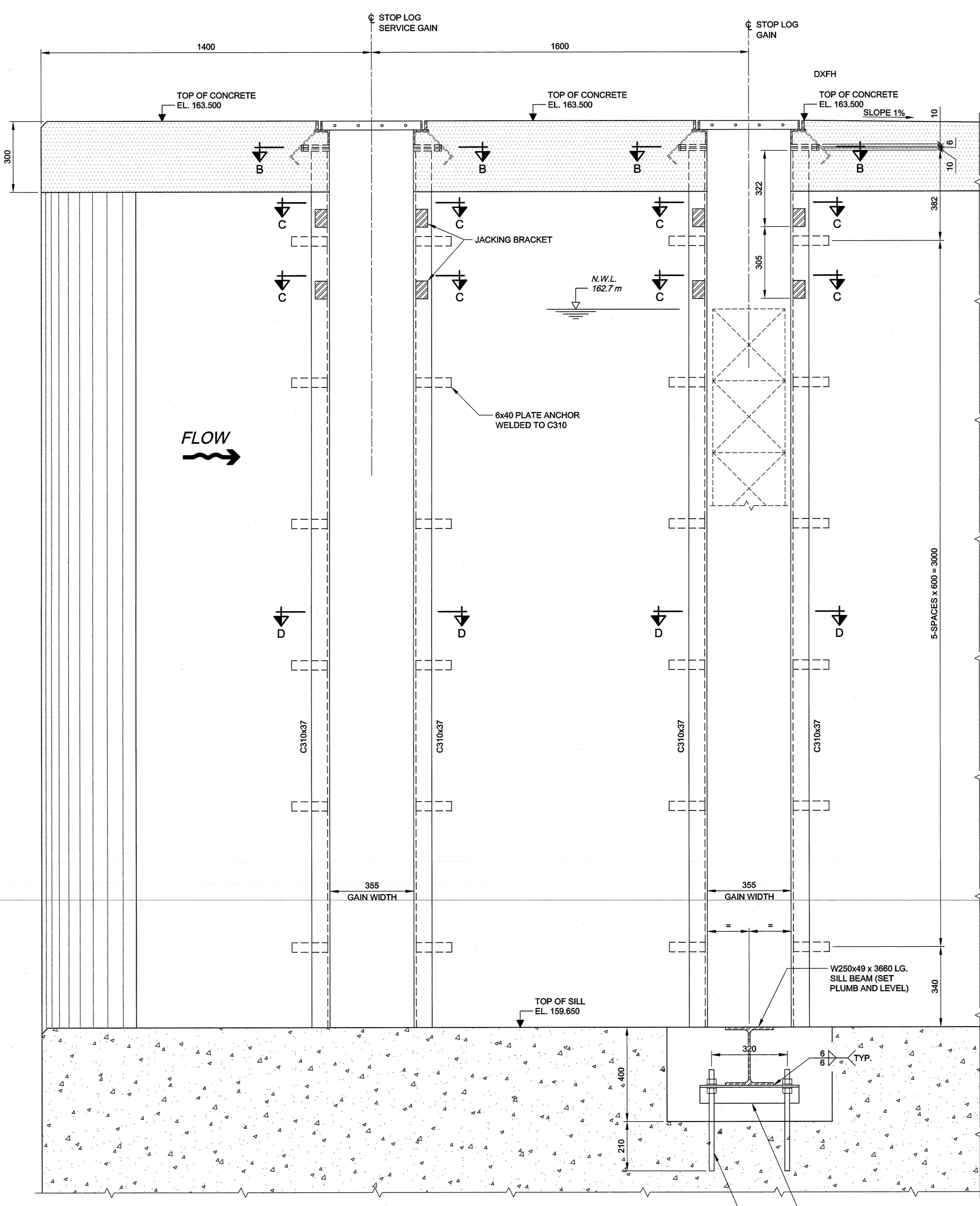
STOP LOG GAINS - ELEVATION 1:10
