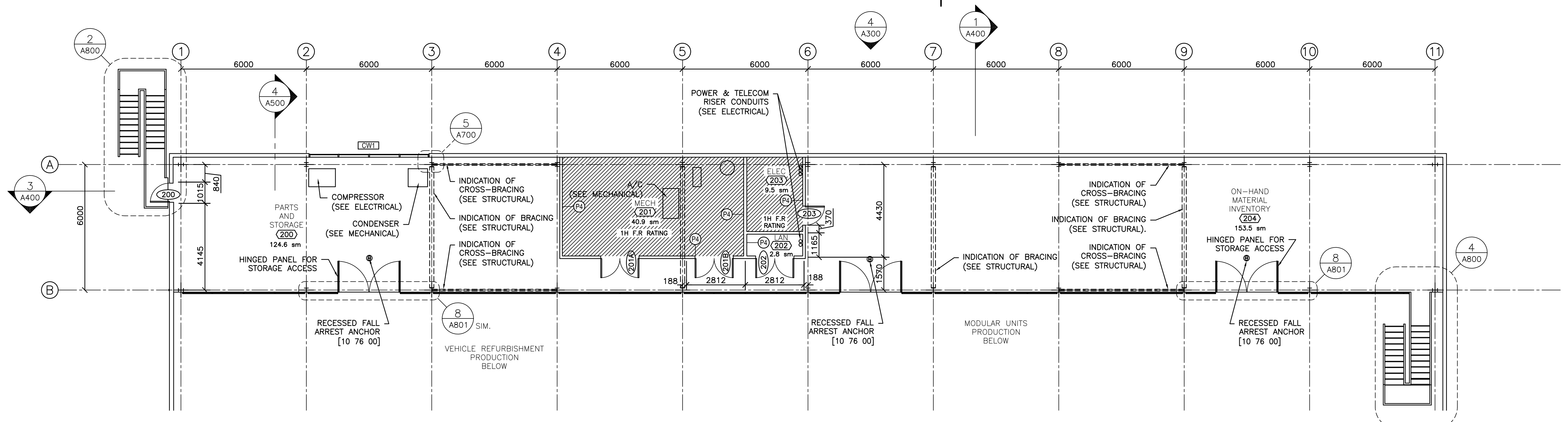
1 MEZZANINE FLOOR PLAN SCALE: 1:100 APPROX. NORTH
