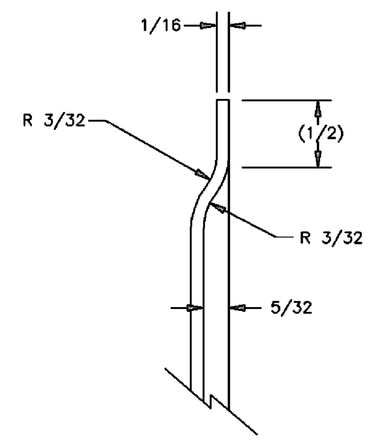
DETAIL A SCALE NTS
