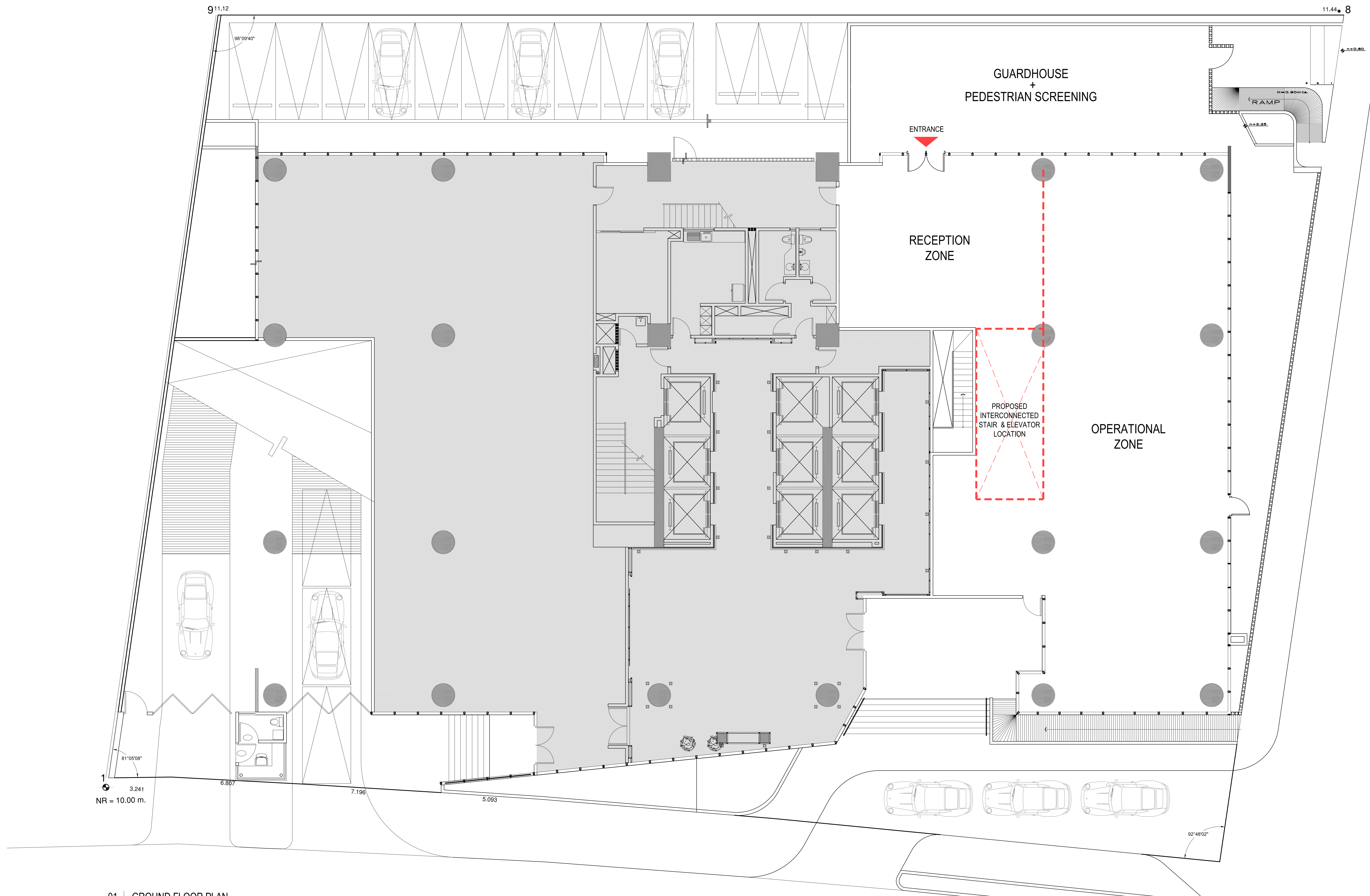
01 | GROUND FLOOR PLAN
