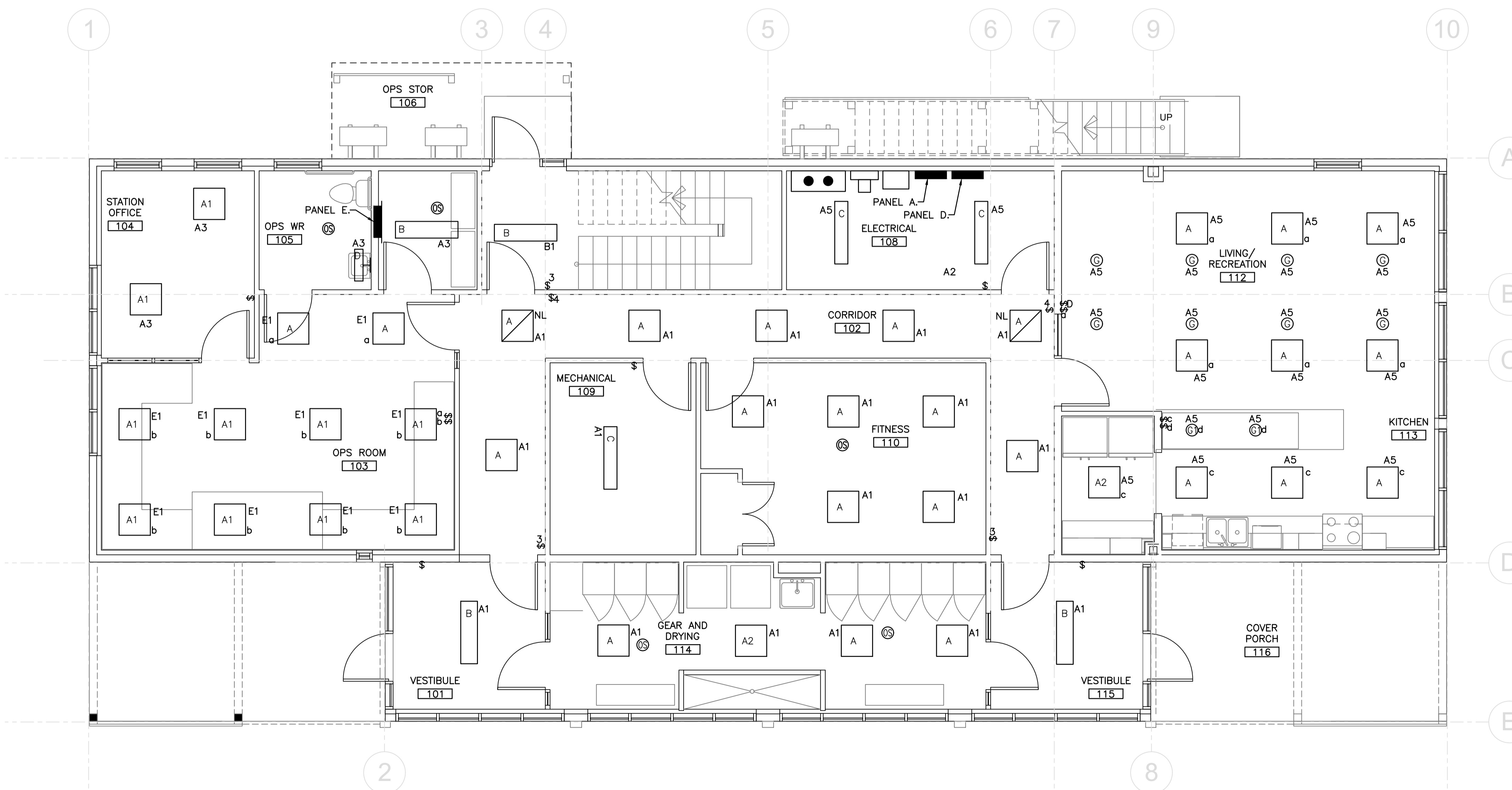
LIGHTING - MAIN BUILDING LEVEL 1
