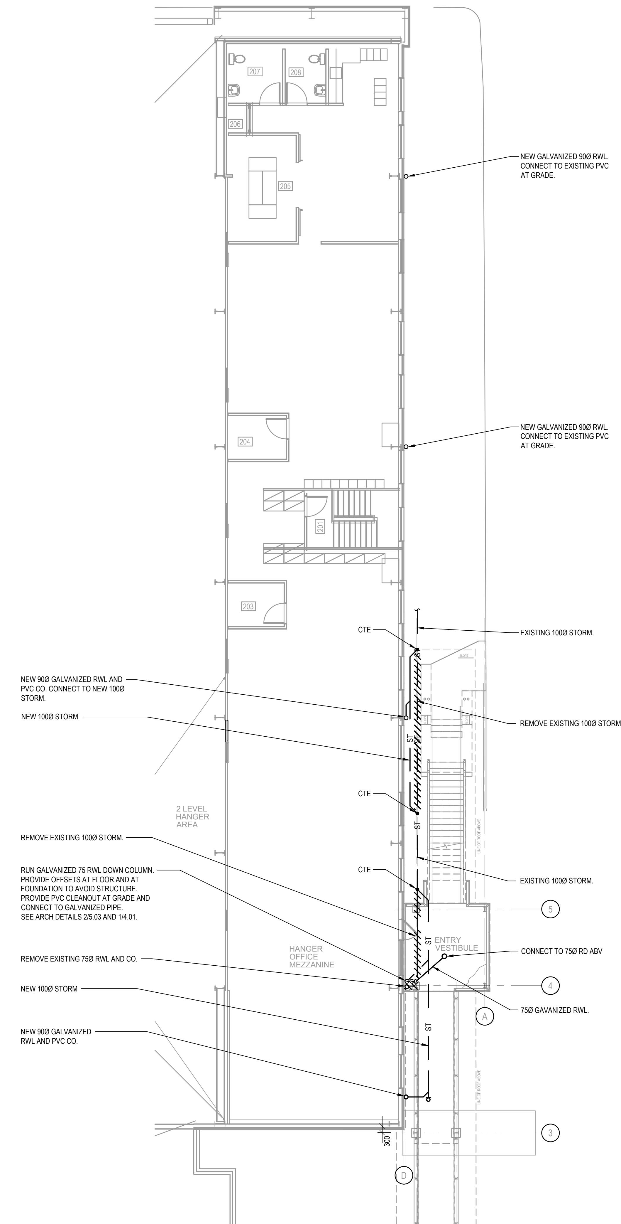
MECHANICAL VESTIBULE AND WALKWAY PLAN - NORTH M-101 SCALE: 1:100
