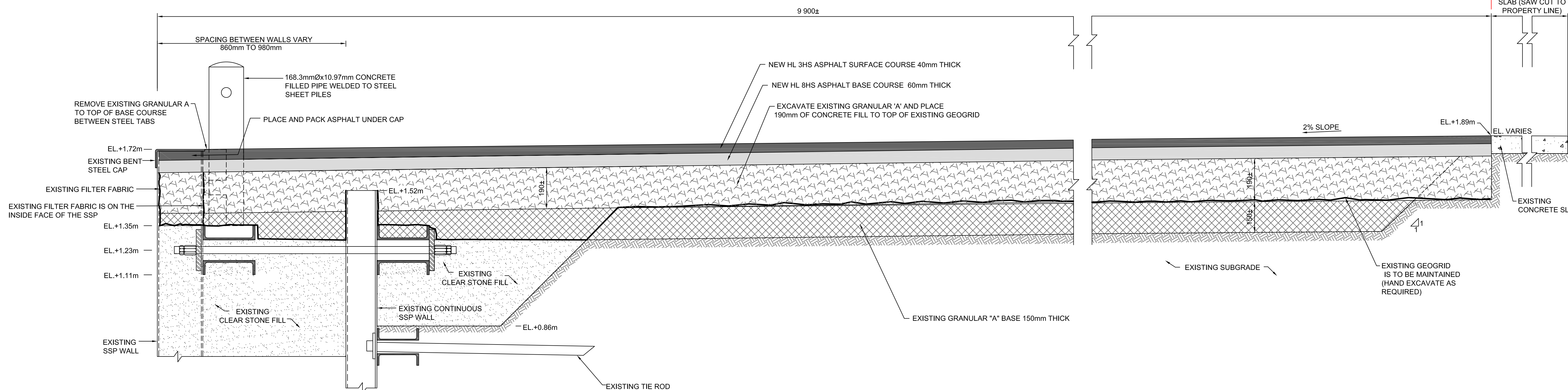
5 TYP. SECTION EXISTING GRAVEL SURFACE (STA. 384.00EP TO 0+386.00EP) SCALE: 1:10
