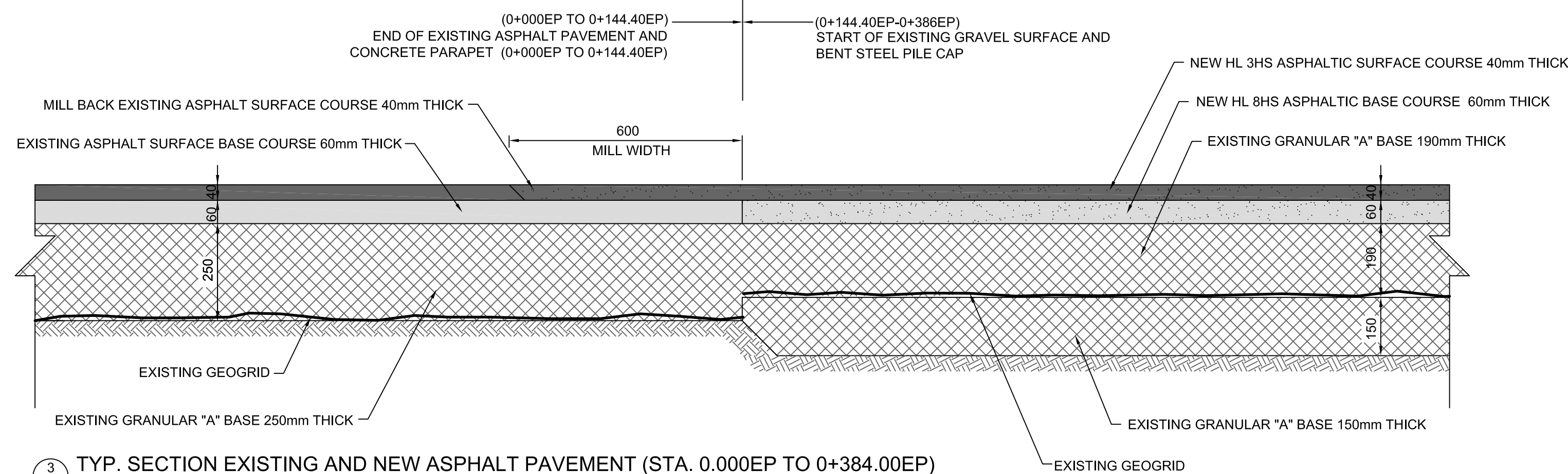
3 TYP. SECTION EXISTING AND NEW ASPHALT PAVEMENT (STA. 0.000EP TO 0+384.00EP) SCALE: 1:10
