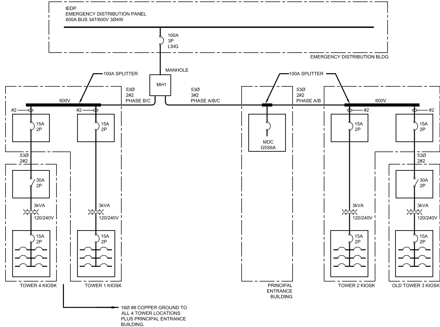
NEW SINGLE LINE DIAGRAM SCALE NTS
