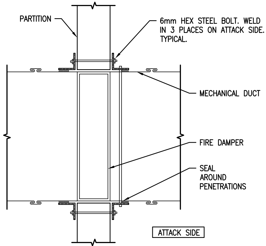
1 SECURE DUCT DETAIL – SECTION 1:10
