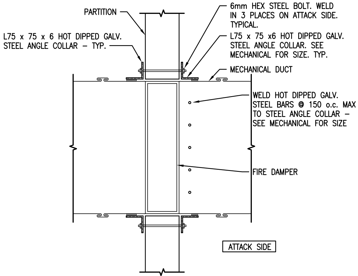
1 SECURE DUCT DETAIL – PLAN VIEW 1:10
