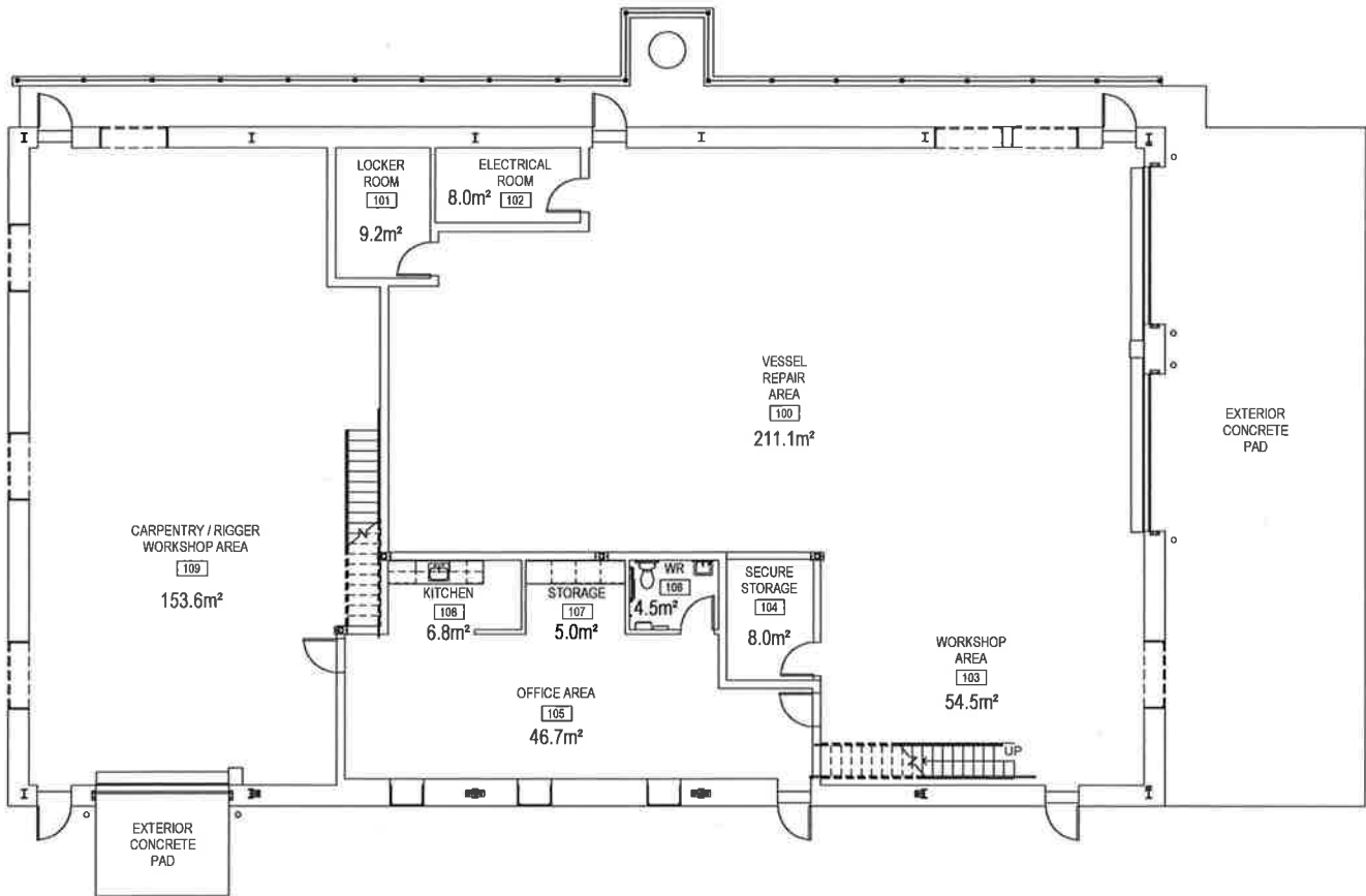
1 LEVEL ONE FLOOR PLAN NTS
