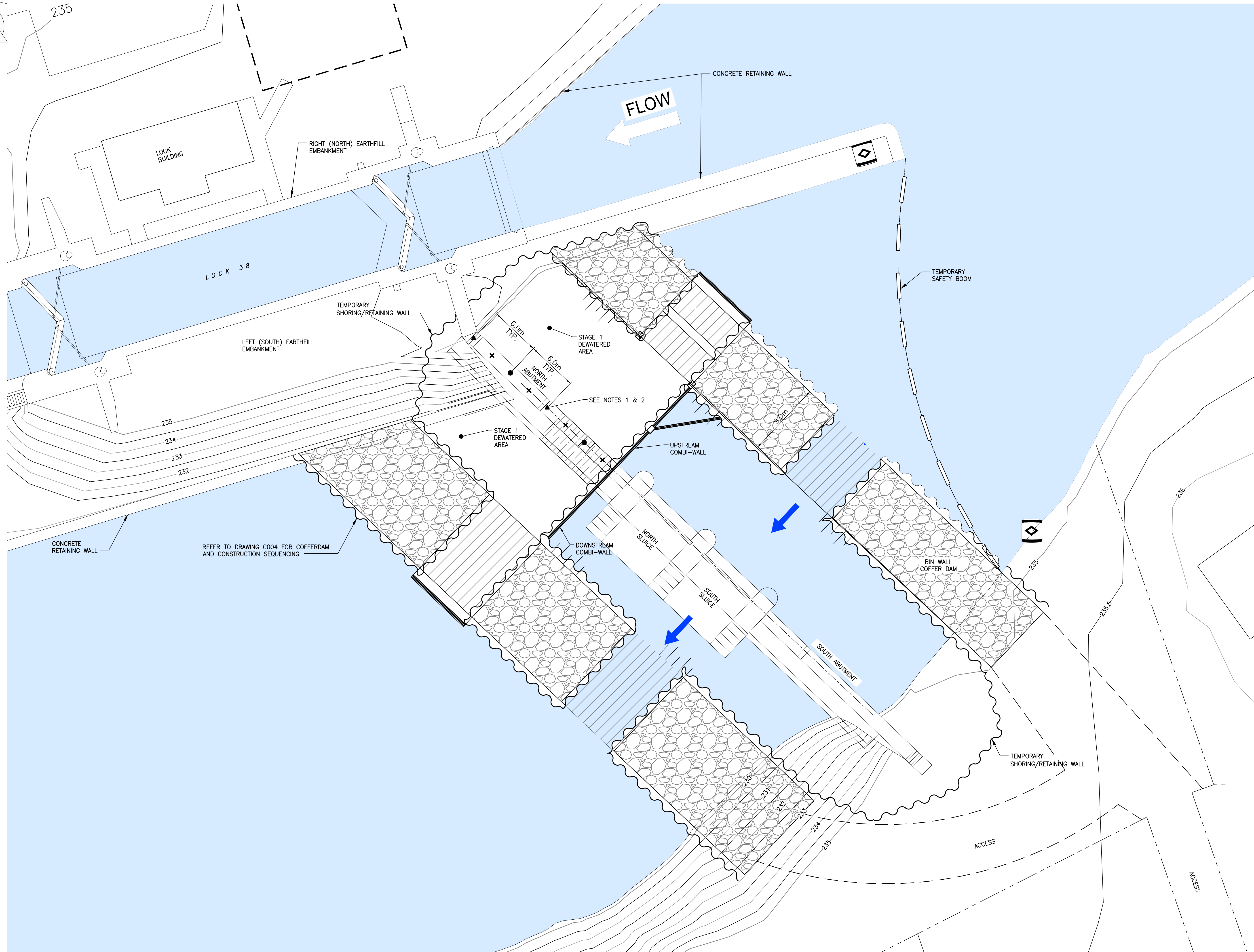
FOUNDATION PREPARATION – STAGE 1 SCALE 1:200 SCALE: 1:200 METRIC 24"x36"
