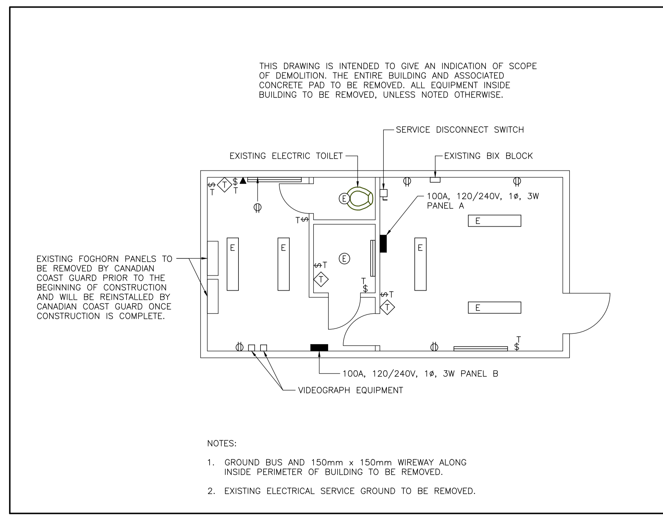
2 DEMOLITION FLOOR PLAN - EQUIPMENT BUILDING E01 1:50
