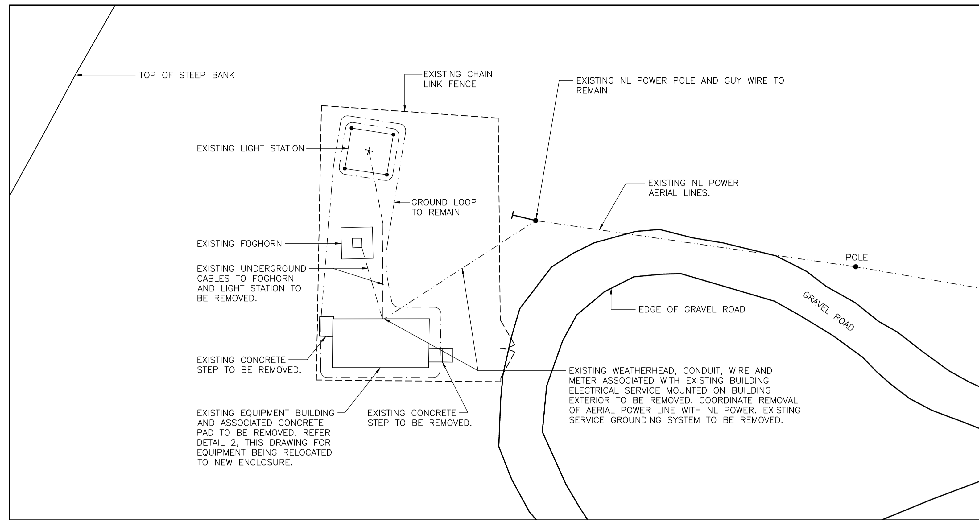
1 DEMOLITION SITE PLAN E01 1:200
