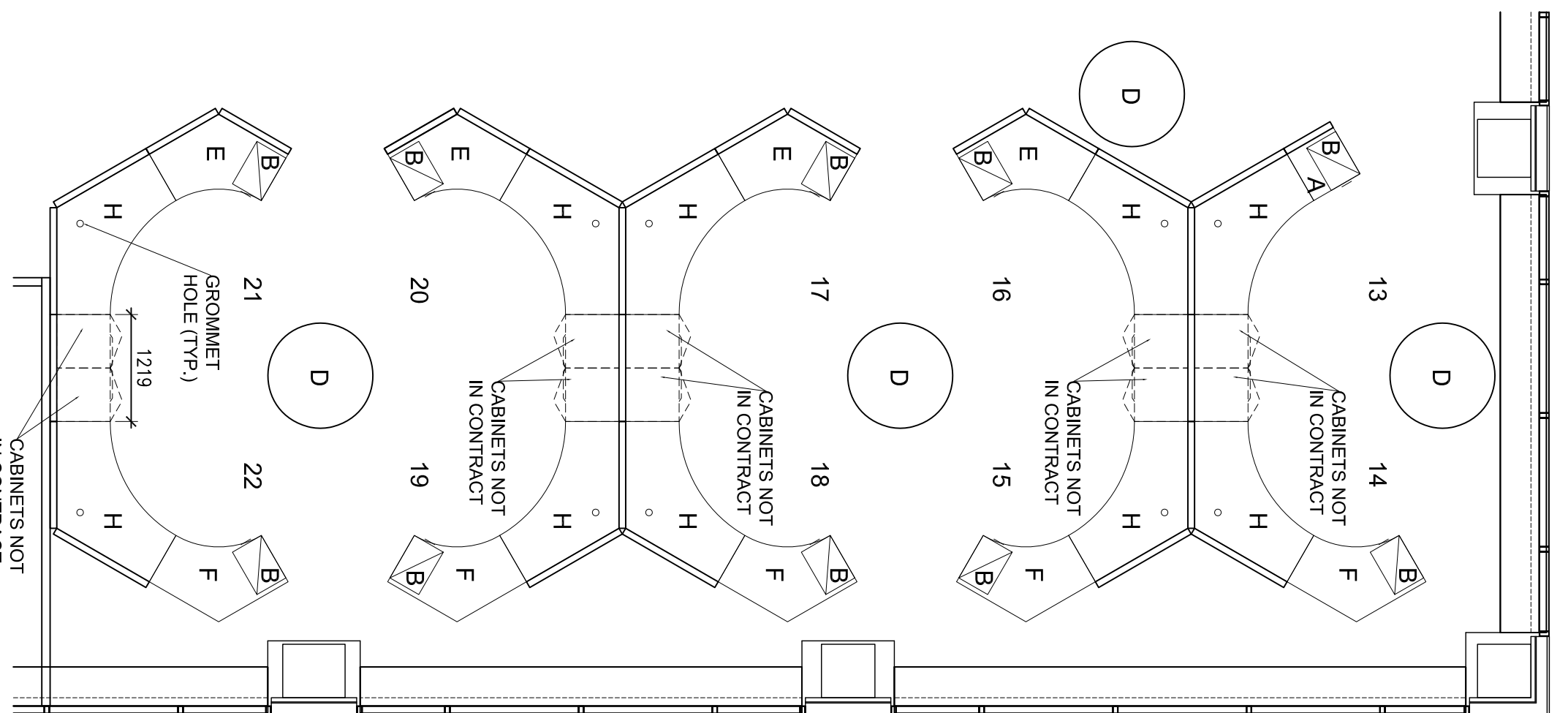
AREA 2 - SURFACE PLAN
