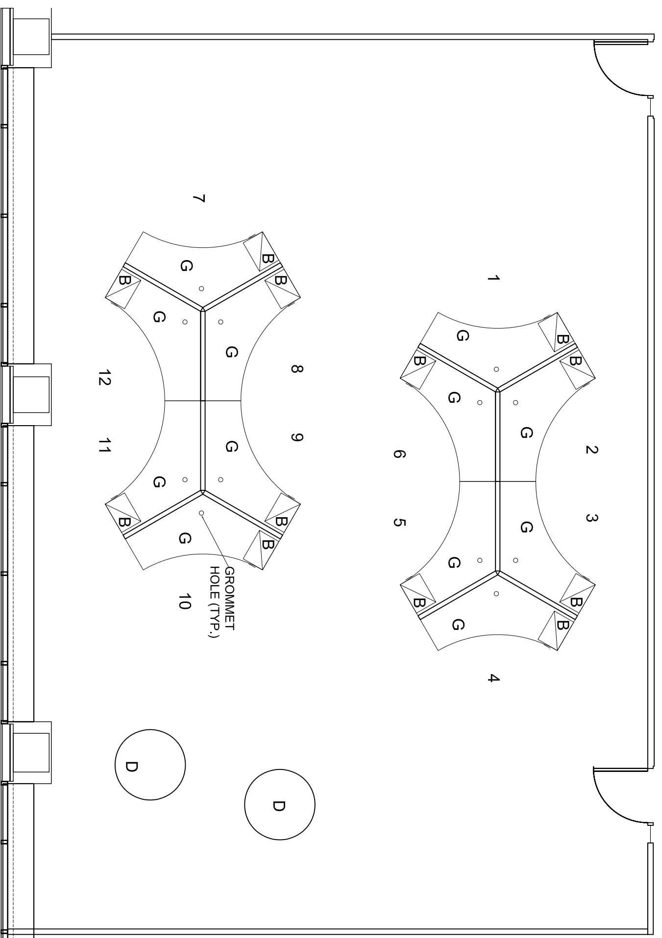
AREA 1 - SURFACE PLAN
