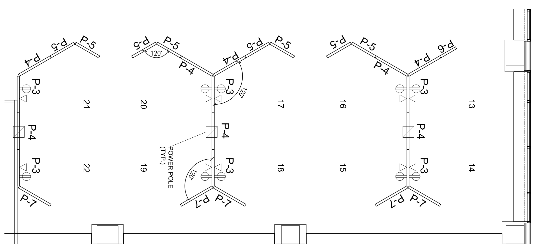
AREA 2 - PANEL PLAN
