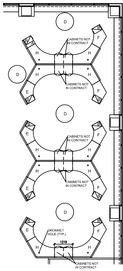
AREA 2 - SURFACE PLAN
