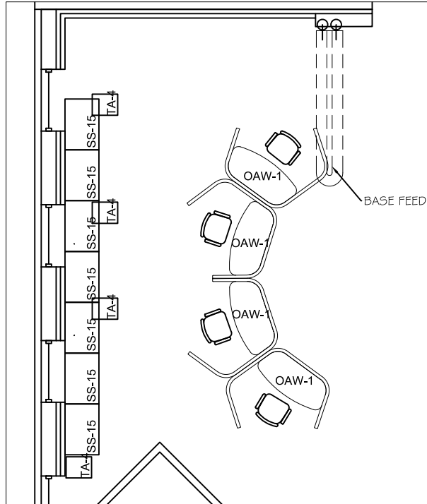
FURNITURE LAYOUT - CB-J
