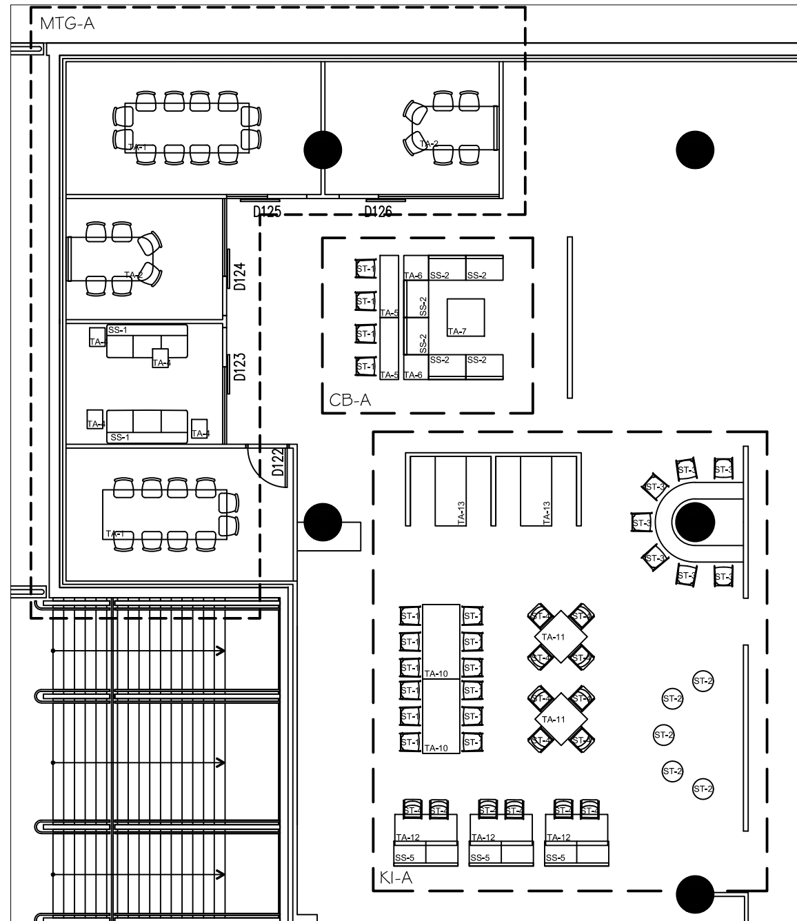
FLOOR PLAN - AREA 1 SCALE: 3/32"=1'-0"
