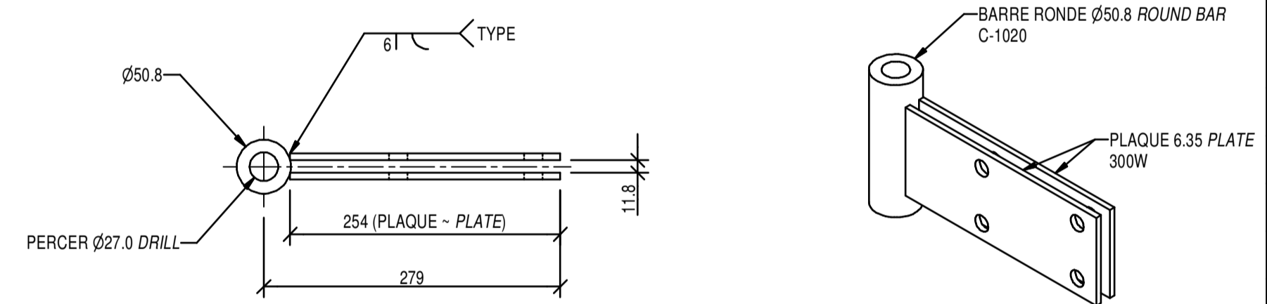
PLAN - TOP
