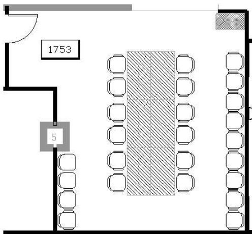
PROPOSED PLAN
