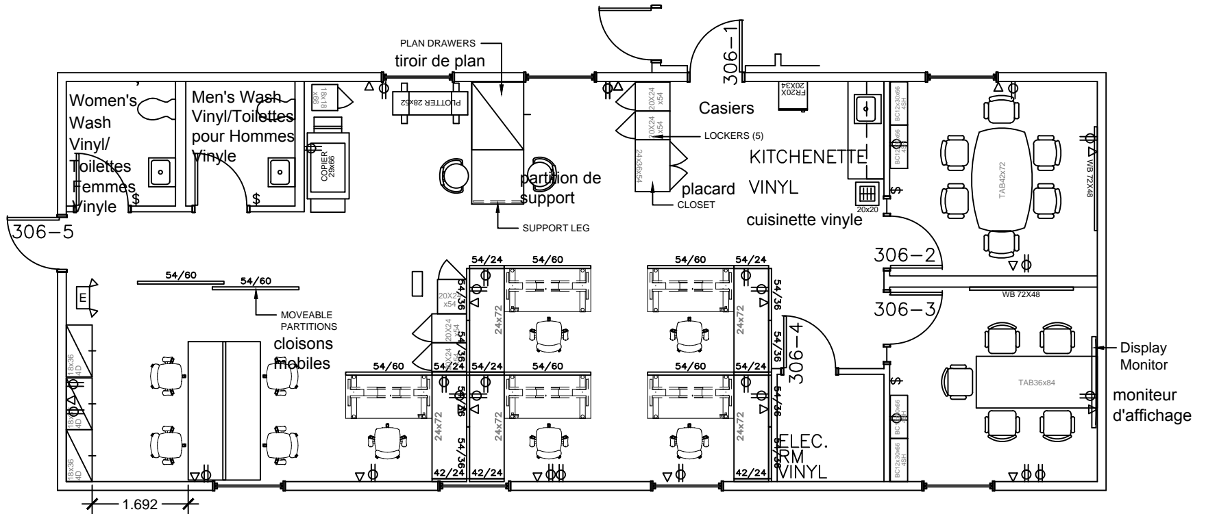
Ground Floor Plan - Proposed (Option 2.x)
