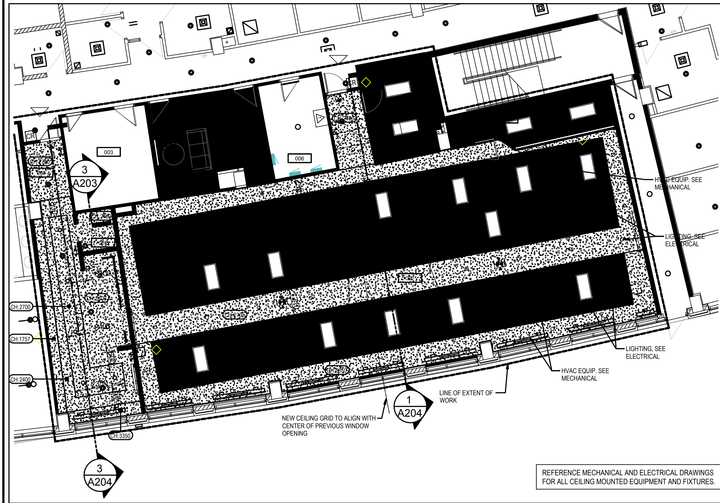
LEVEL 1_NEW REFLECTED CEILING PLAN
