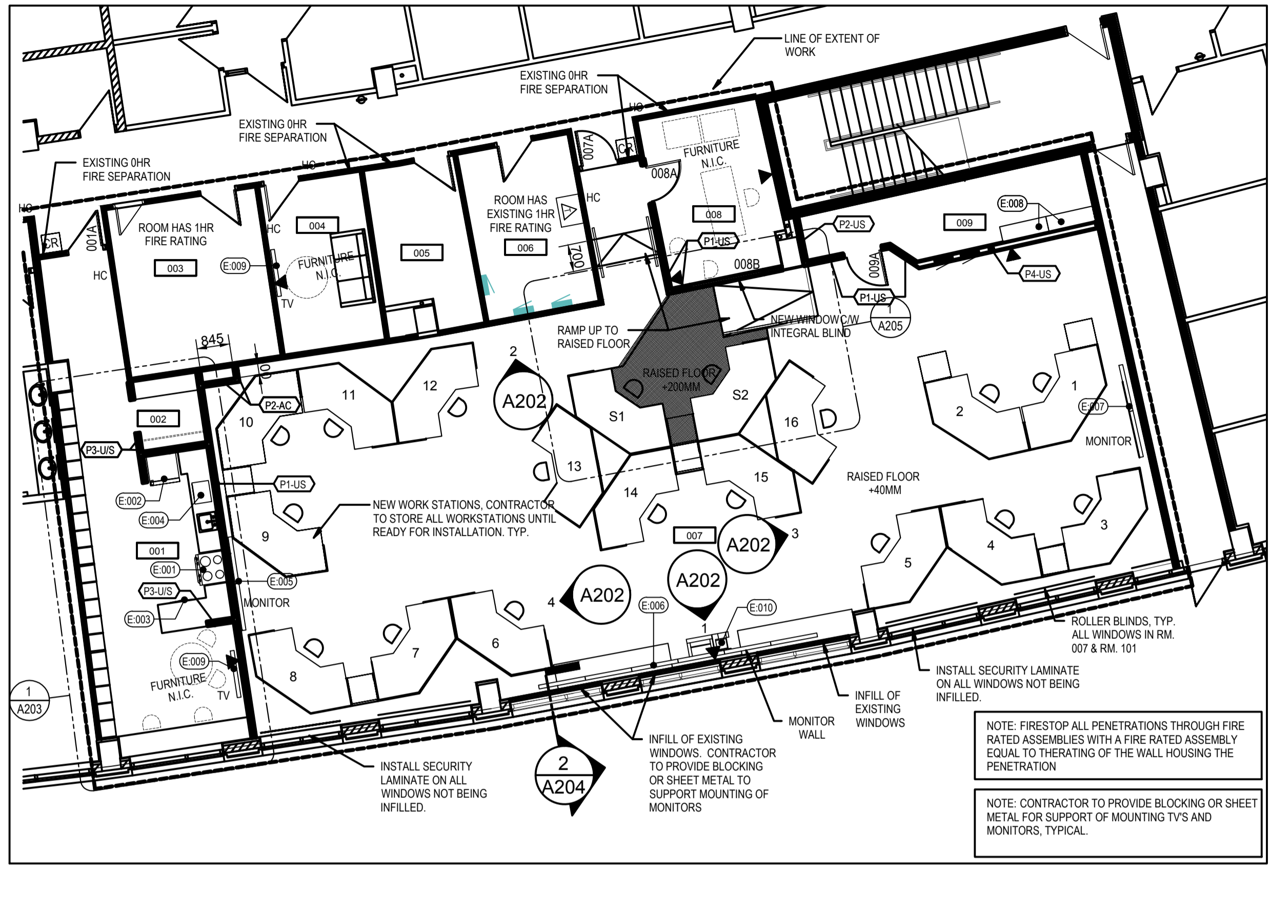
LEVEL 1_NEW GENERAL FLOOR PLAN
