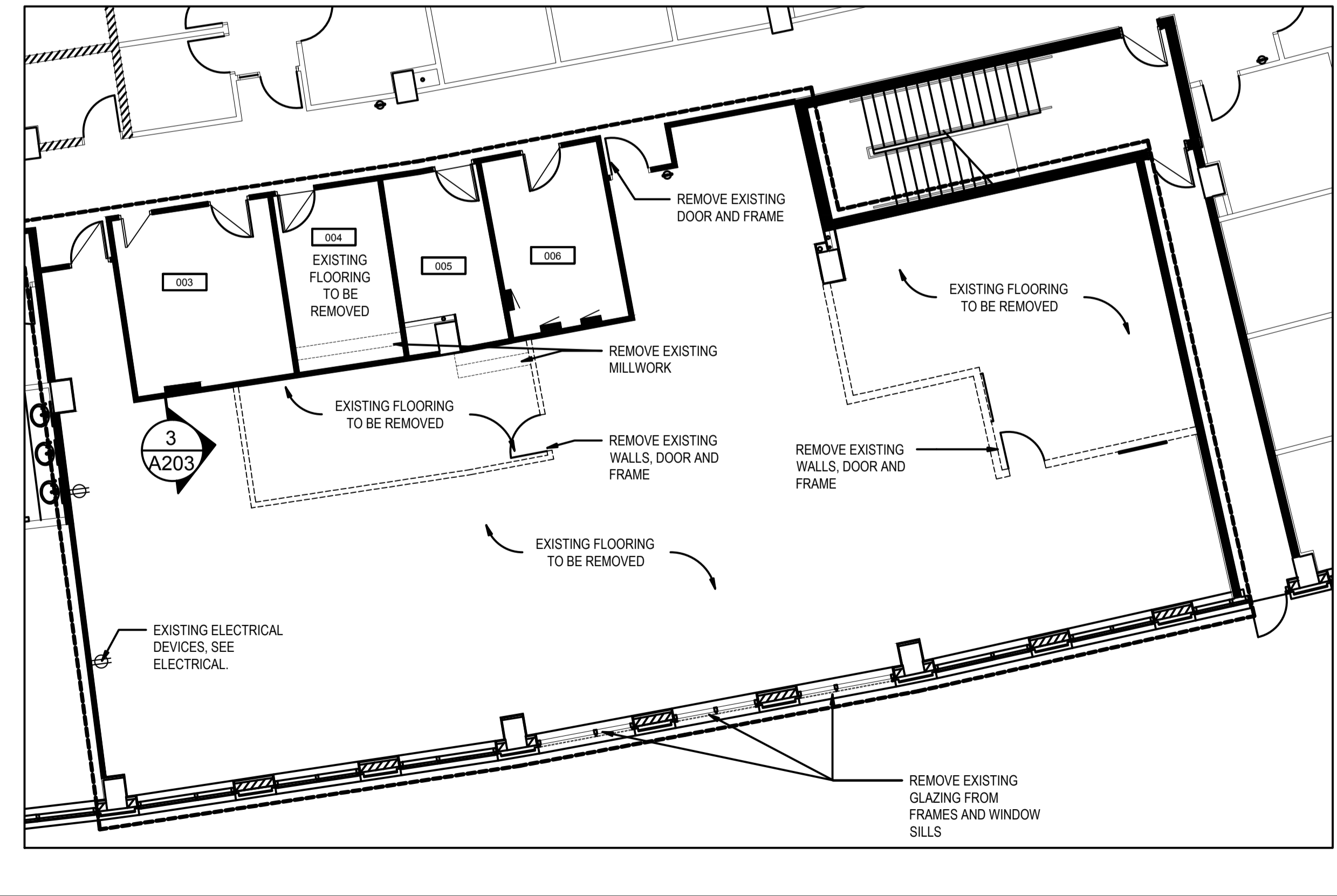
LEVEL 1_EXISTING / DEMO FLOOR PLAN
