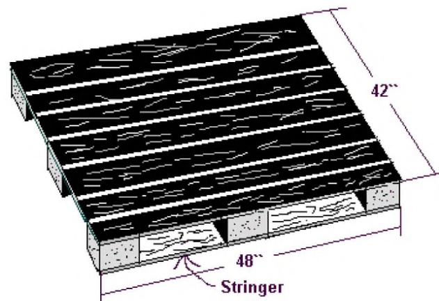
Stringer - SOLID BLOCKS - 4" X 6" X 3" High
