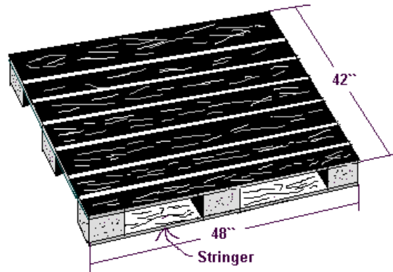
Stringer - SOLID BLOCKS - 4" X 6" X 3" High
