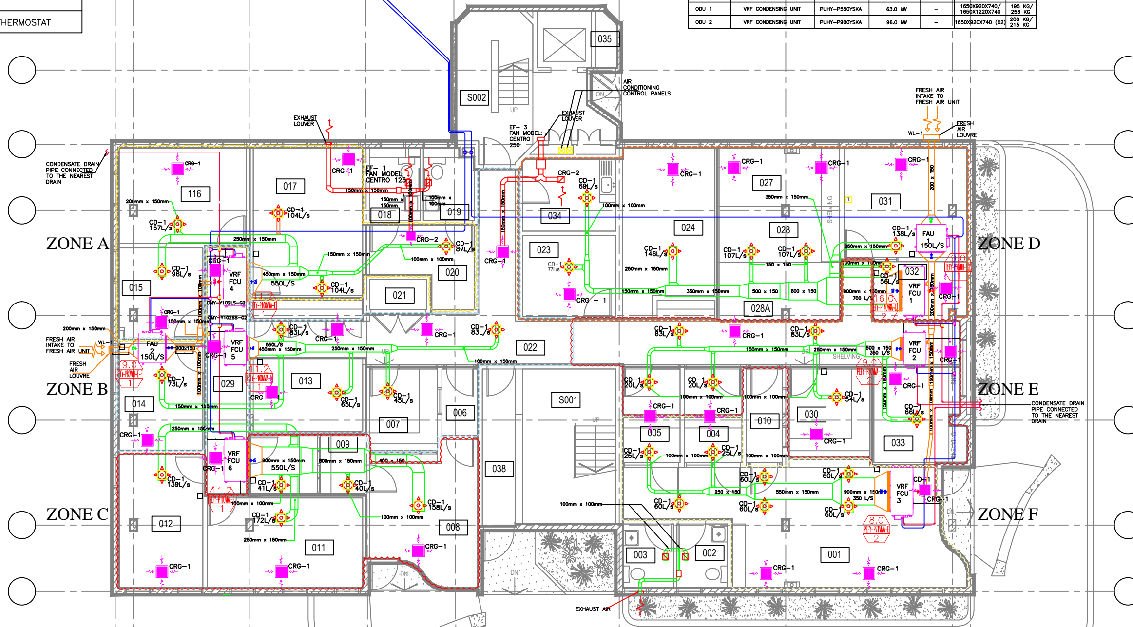
GROUND FLOOR PLAN - AIRCONDITIONING AND VENTILATION SYSTEM 1 : 125
