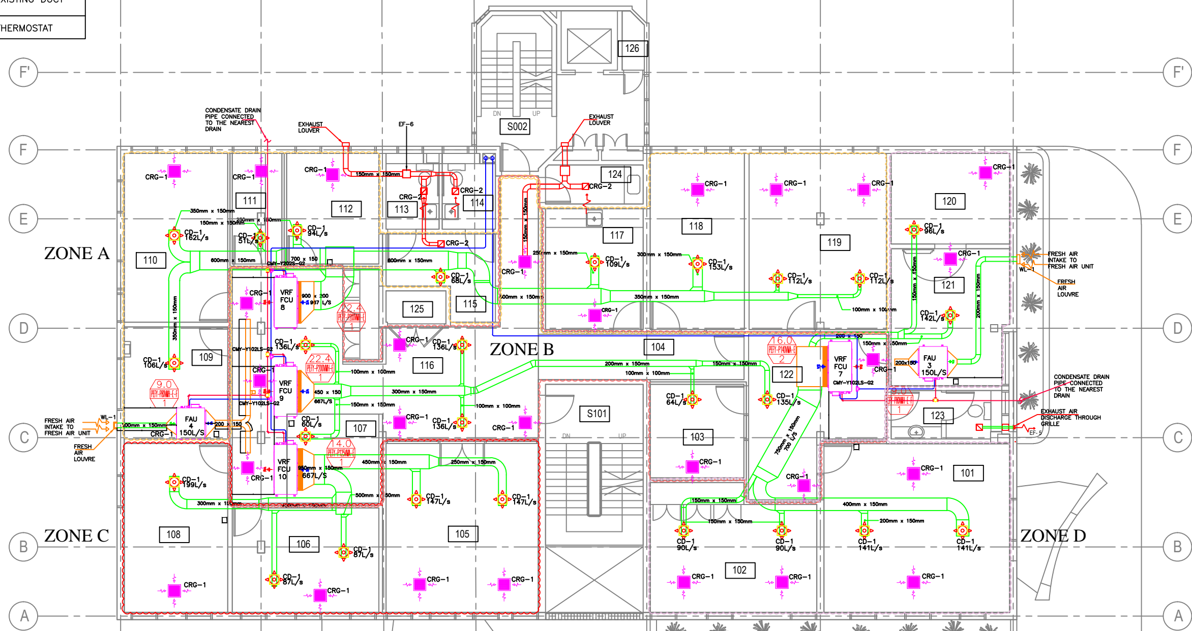
FIRST FLOOR PLAN - AIRCONDITIONING AND VENTILATION SYSTEM 1 : 125
