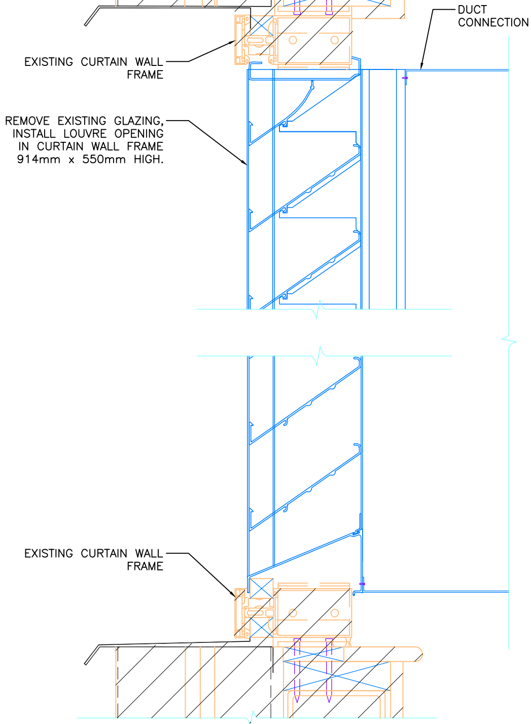
1 VERTICAL SECTION THROUGH NEW LOUVRE A-DT001 SCALE 1:5
