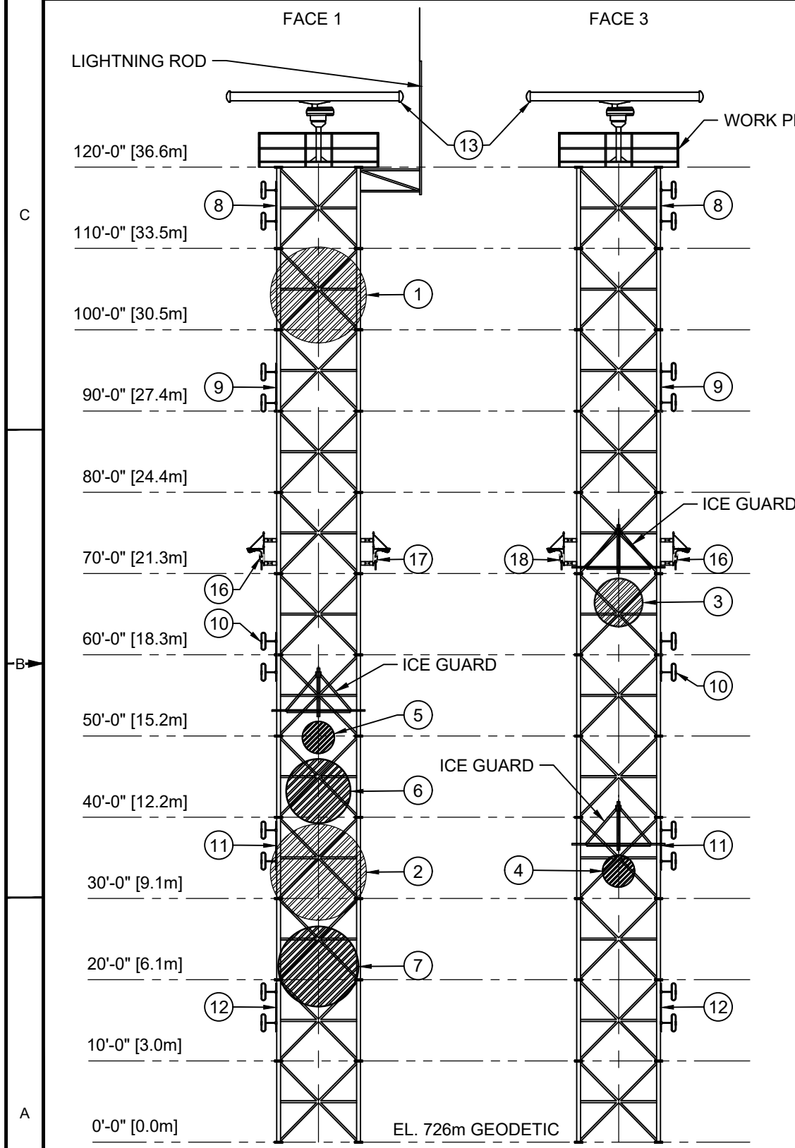
TOWER ELEVATION SCALE 1:200
