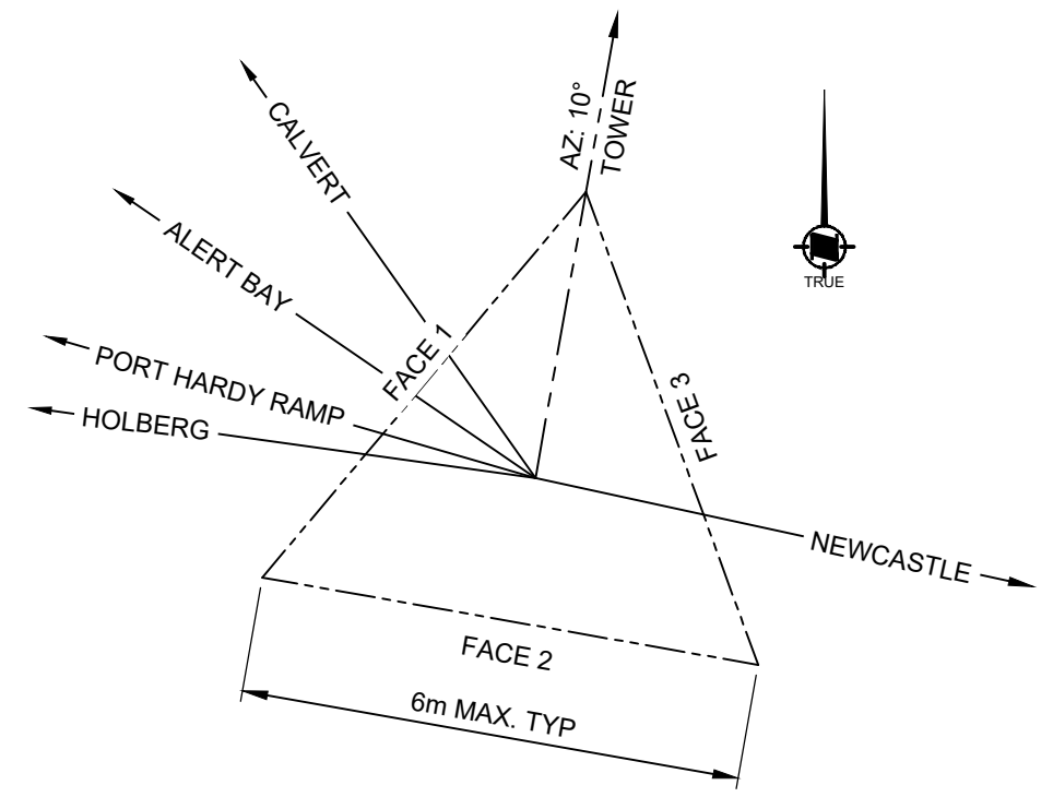
PLAN VIEW SCALE 1:50
