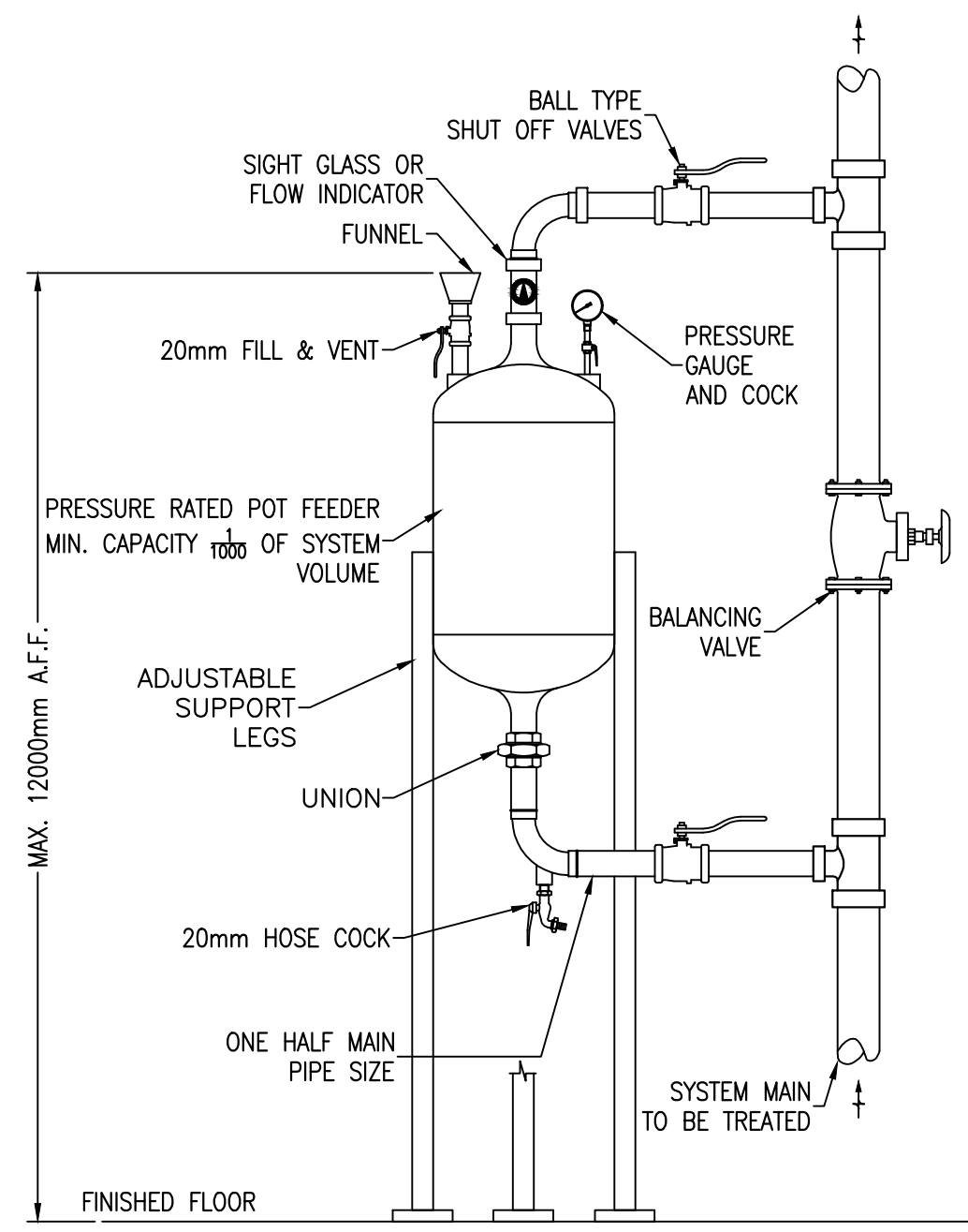
CHEMICAL POT FEEDER DETAIL SCALE : NTS
