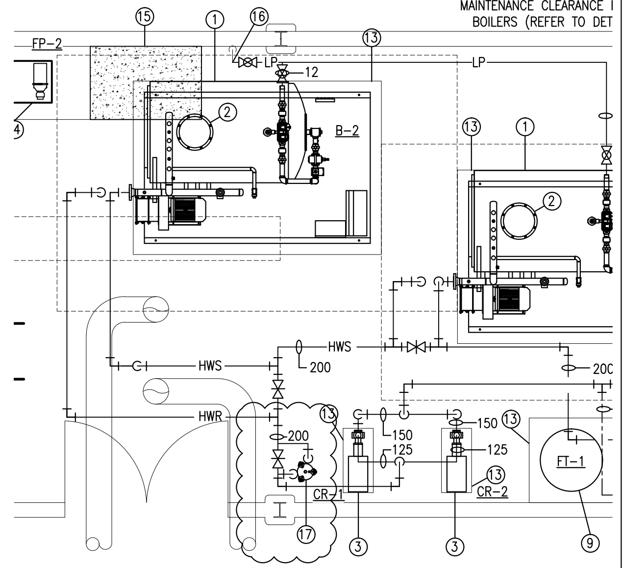
BOILER ROOM PLAN BOILER PIPING NEW LAYOUT SCALE : 1:50
