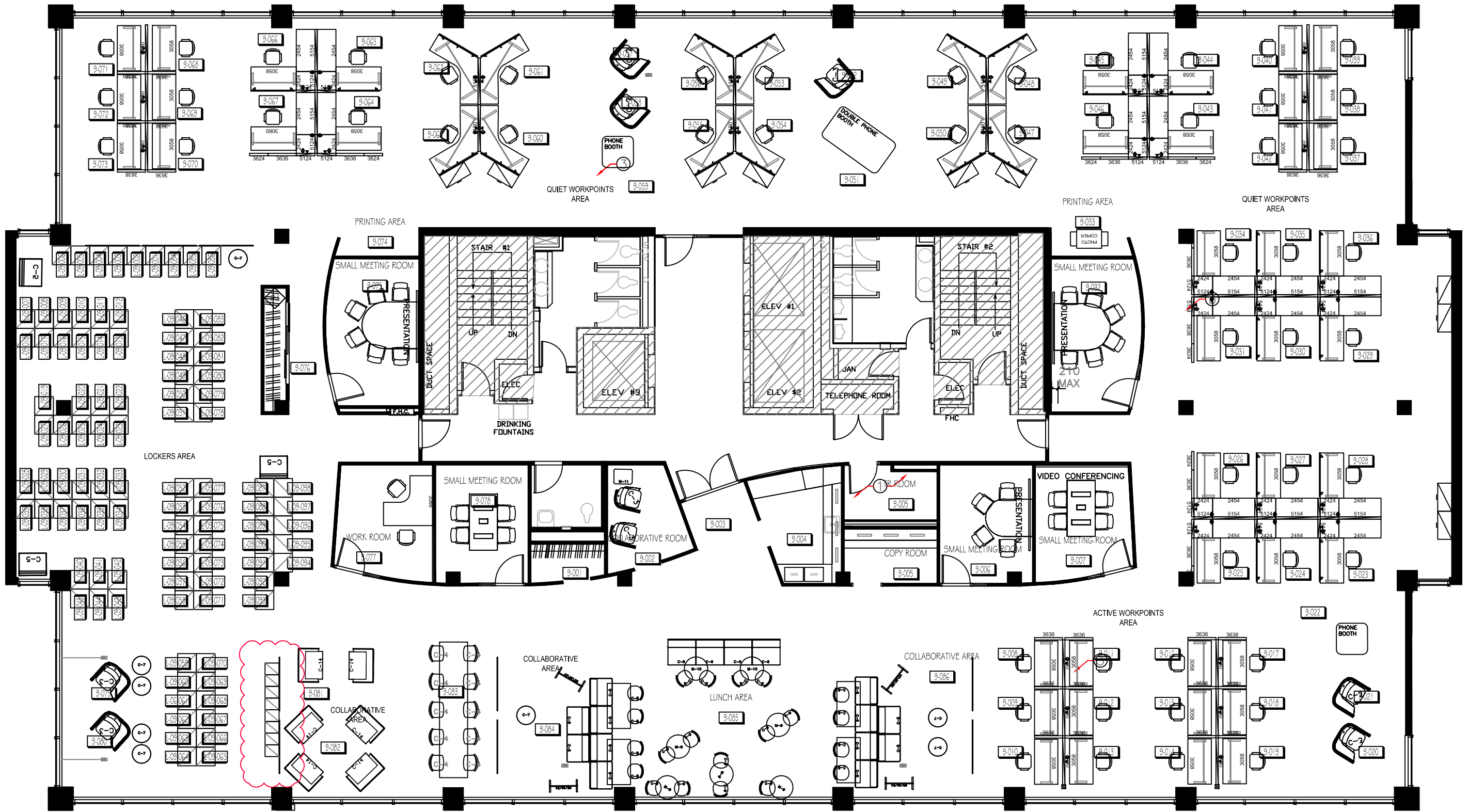
9TH FLOOR — 360 LISGAR SQUARE METER: 116.4 M2
