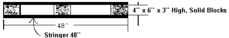
Stringer - SOLID BLOCKS - 4" X 6" X 3" High
