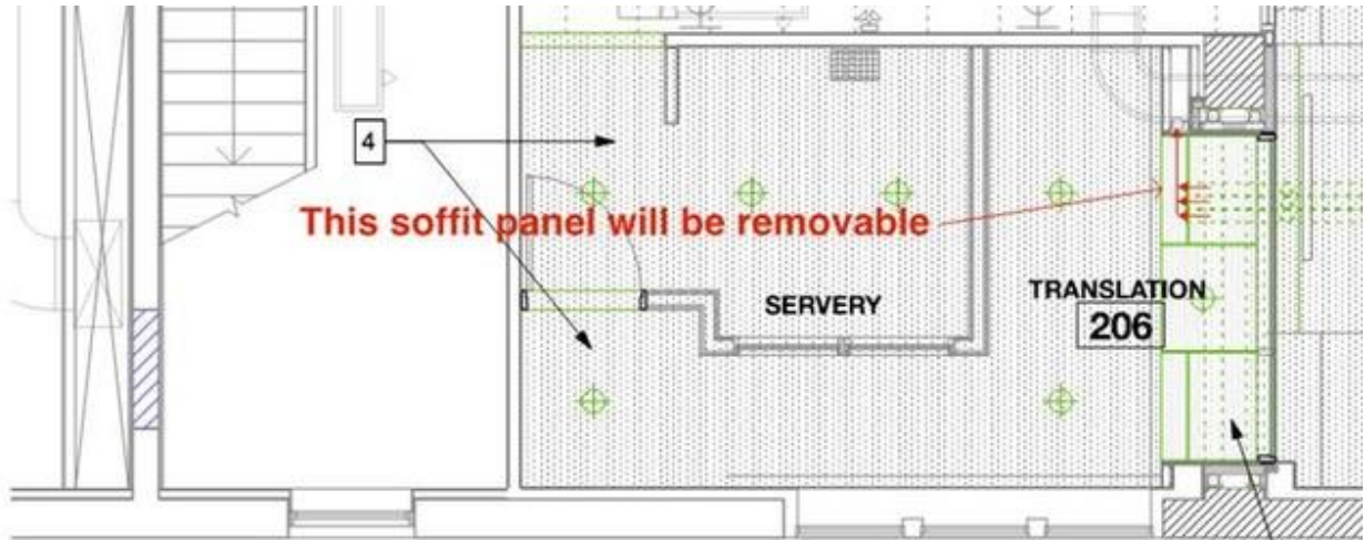
2 PROPOSED REFLECTED CEILING PLAN A-103 Scale: 1:50
