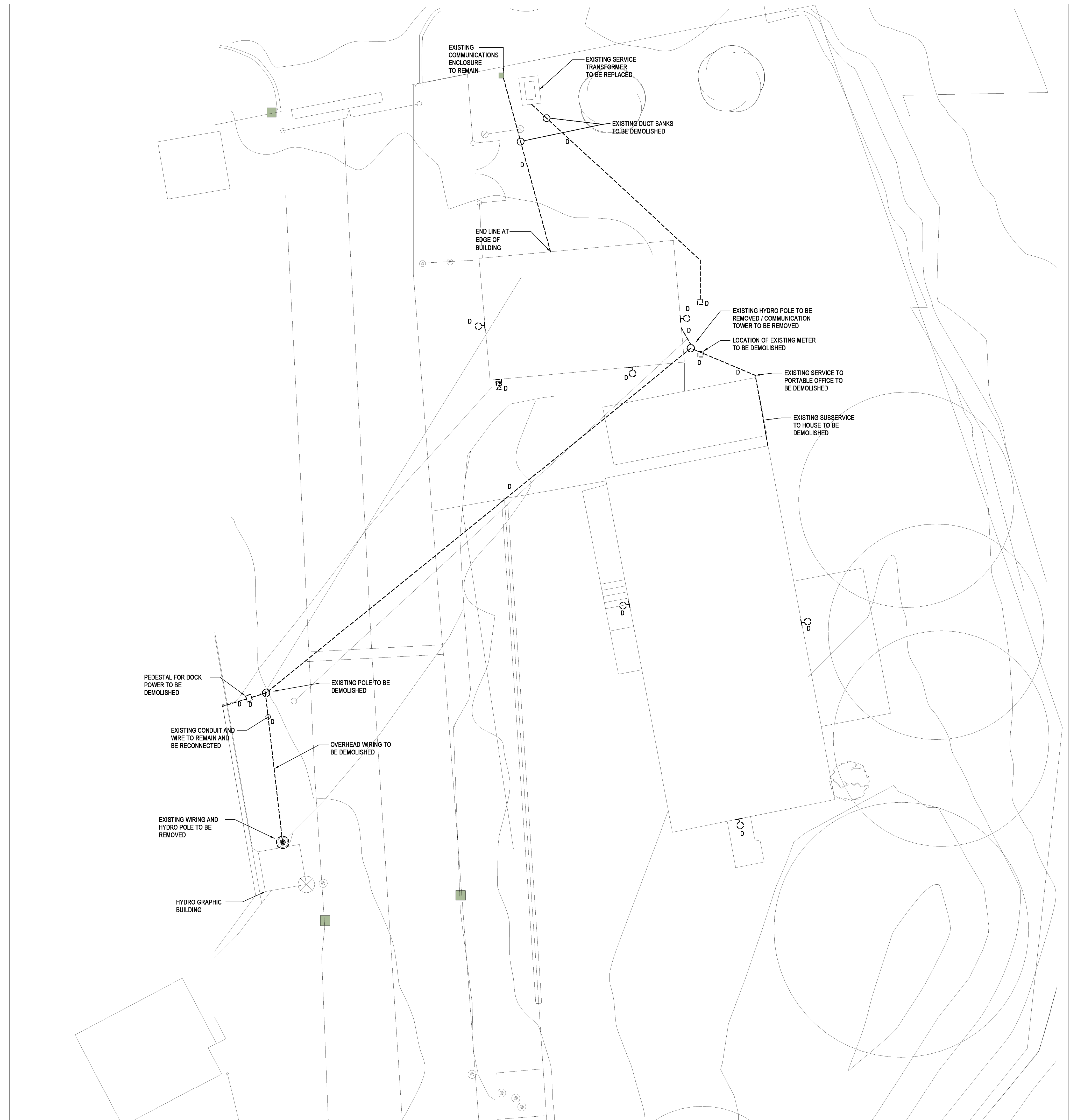
1 ELECTRICAL DEMOLITION POWER SITE PLAN LAYOUT 1 : 100 0 1 2 3 4 5 2 1 SCALE 1:100
