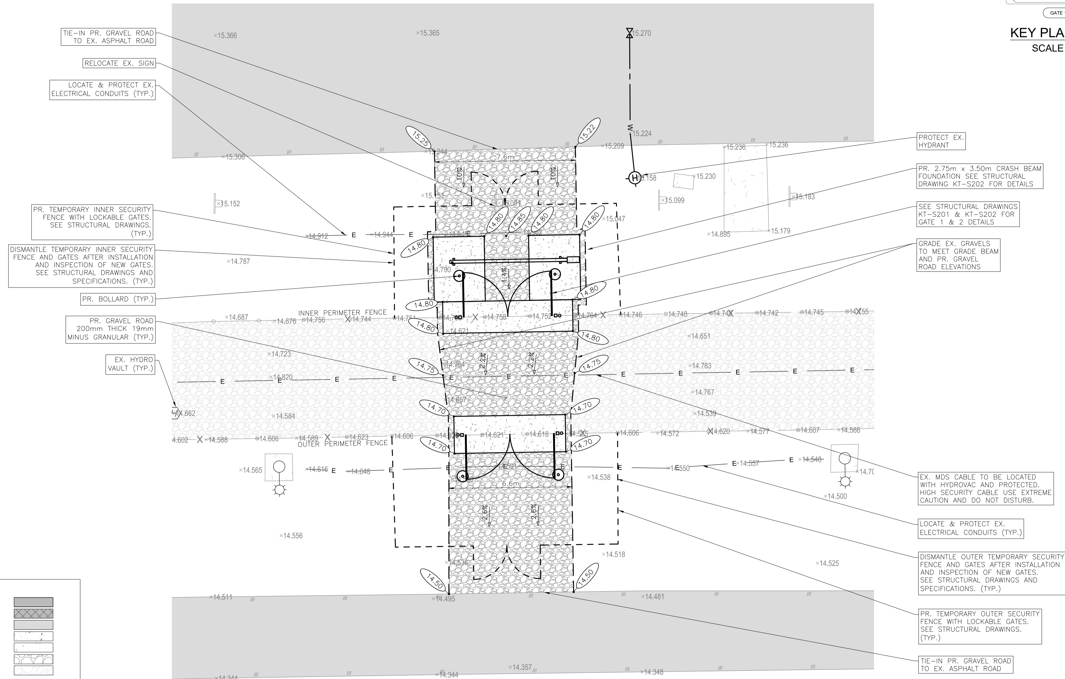
GATES 1 & 2 SCALE 1:100
