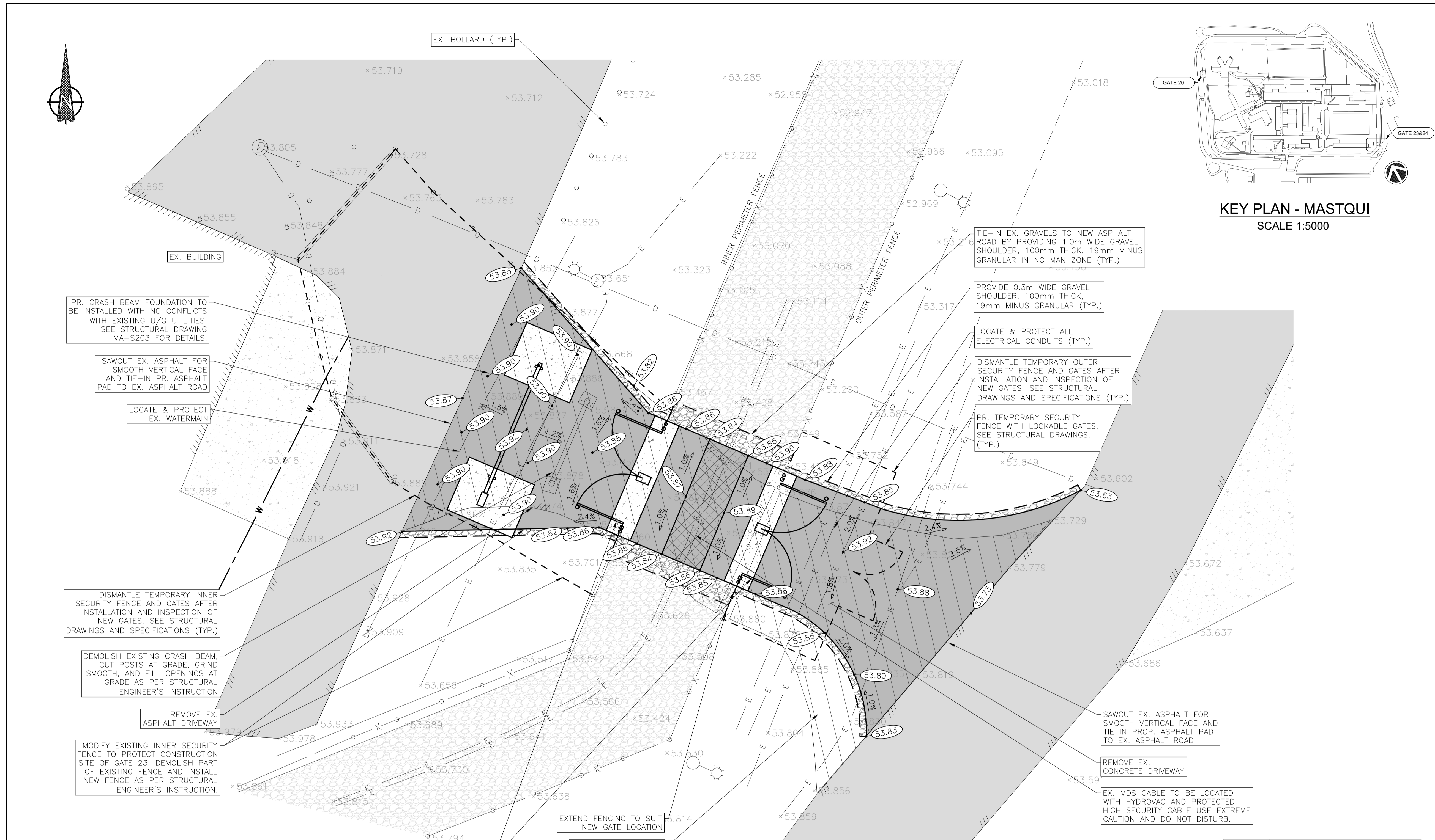
GATES 23 & 24 SCALE 1:100
