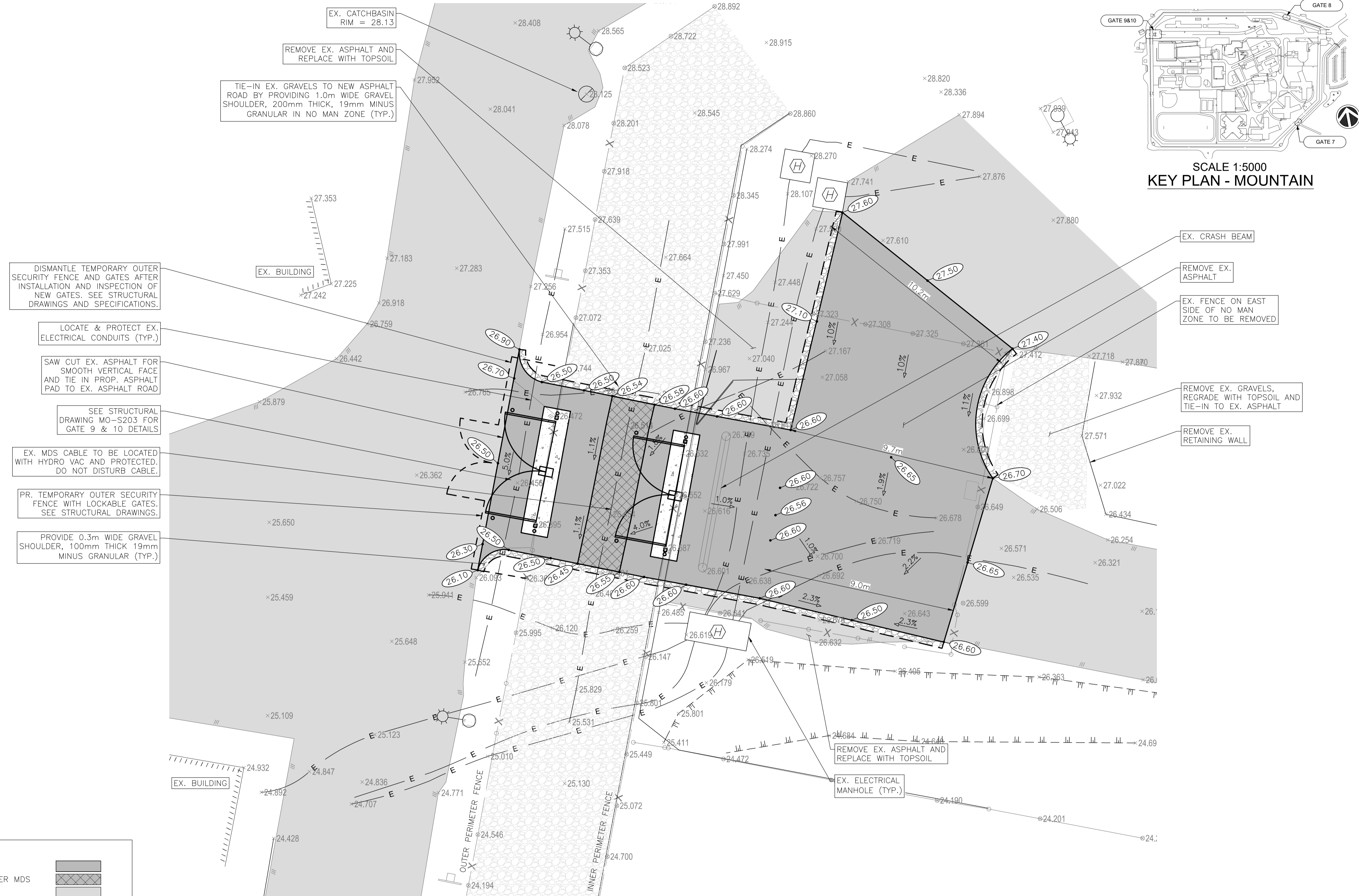
GATE 9 & 10 SCALE 1:100
