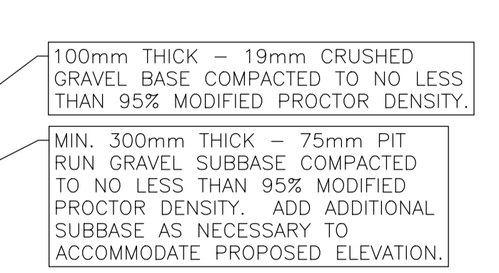
TYPICAL ASPHALT PAVEMENT STRUCTURE SCALE: NTS
