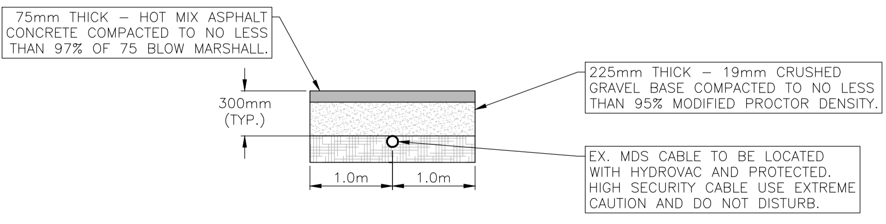
ASPHALT PAVEMENT STRUCTURE OVER MDS CABLE SCALE: NTS
