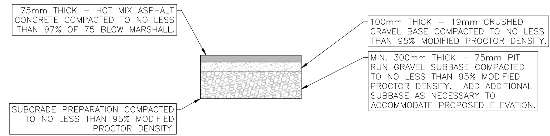
TYPICAL ASPHALT PAVEMENT STRUCTURE SCALE: NTS
