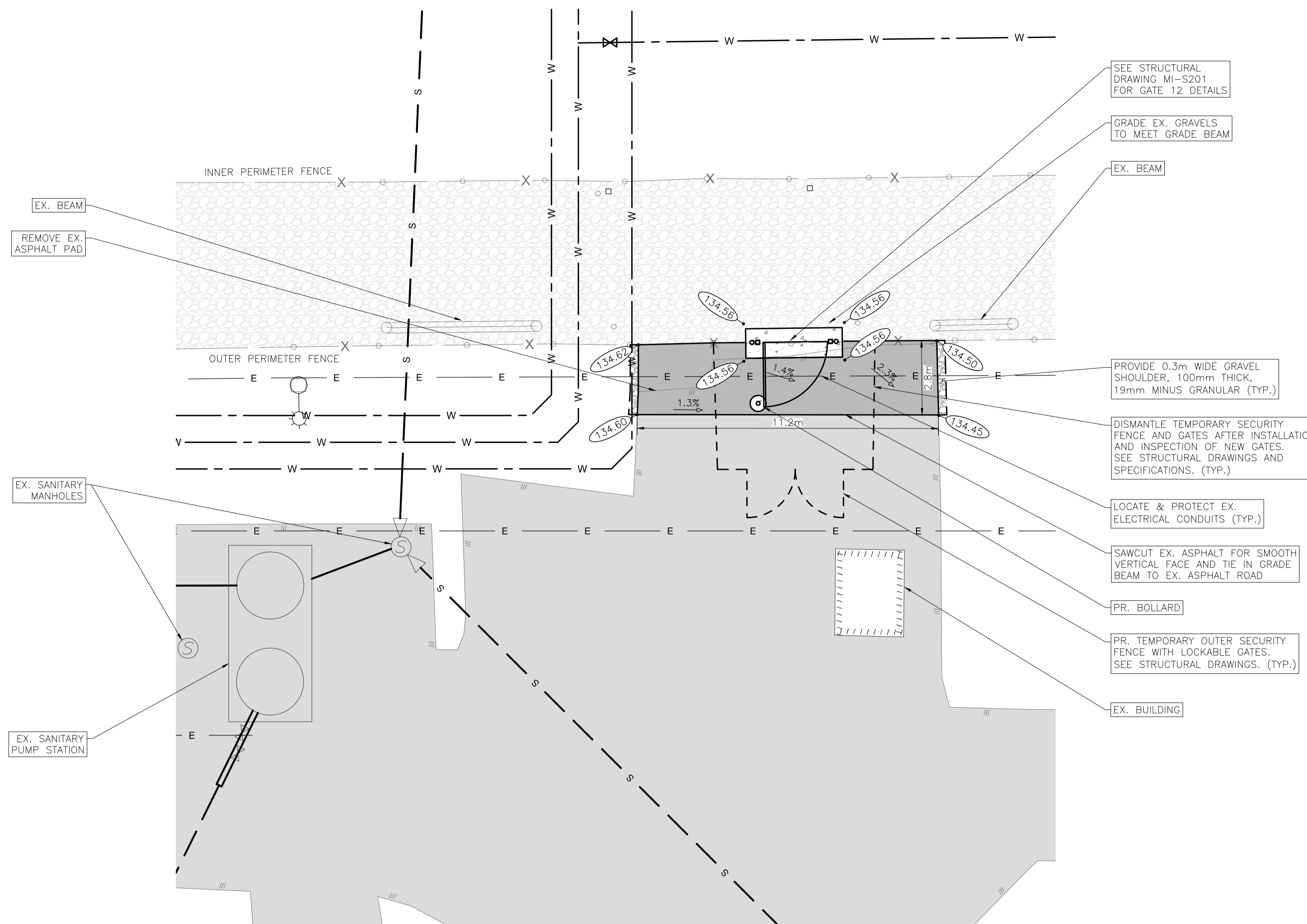
GATE 12 SCALE 1:100
