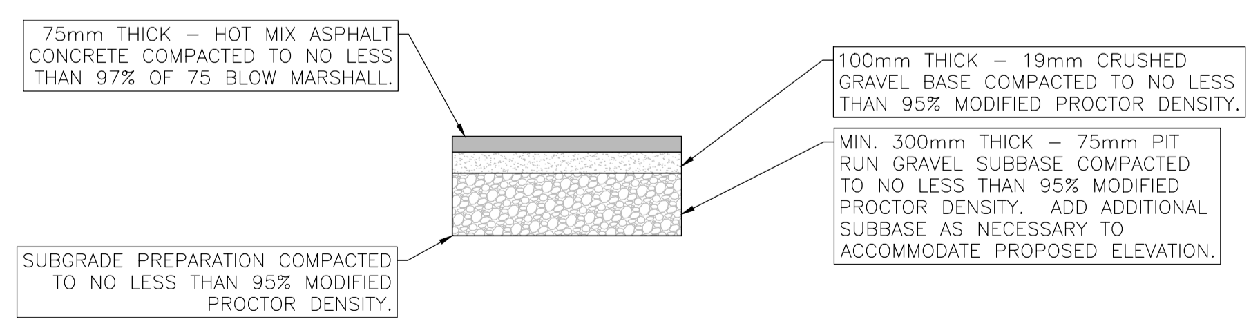
TYPICAL ASPHALT PAVEMENT STRUCTURE SCALE: NTS
