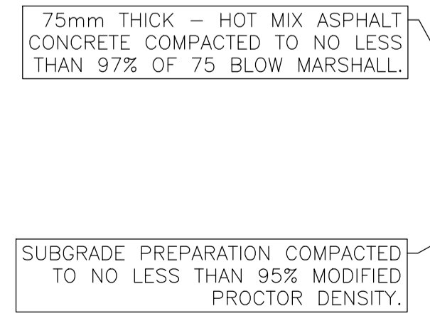
TYPICAL ASPHALT PAVEMENT STRUCTURE SCALE: NTS
