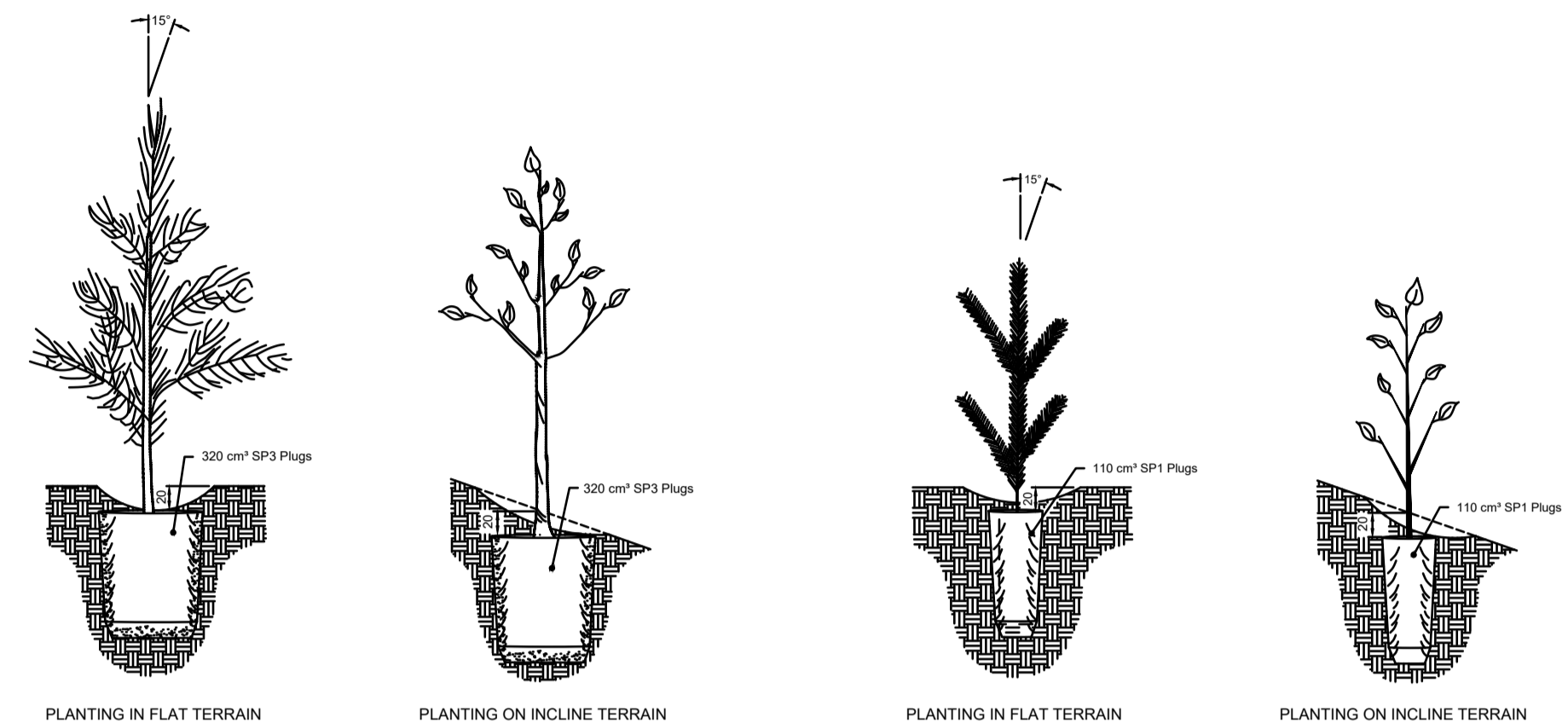
MULTICELL PLUGS PLANTING DETAIL
