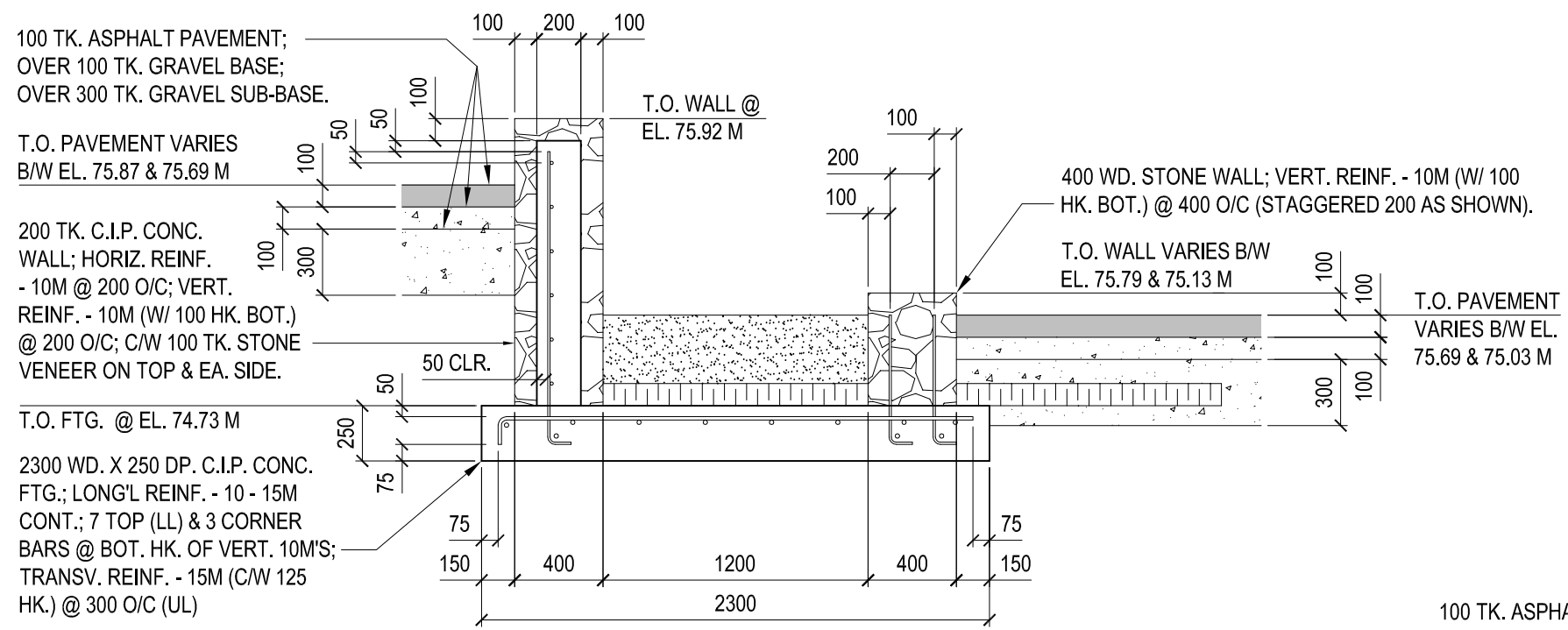
1 X-SECTION THRU. STONE WALL PLANTER. S13 SCALE - 1 : 30
