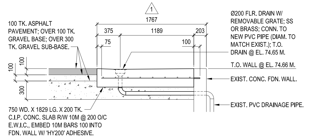
2 X-SECTION THRU. STORM DRAIN. S13 SCALE - 1 : 30
