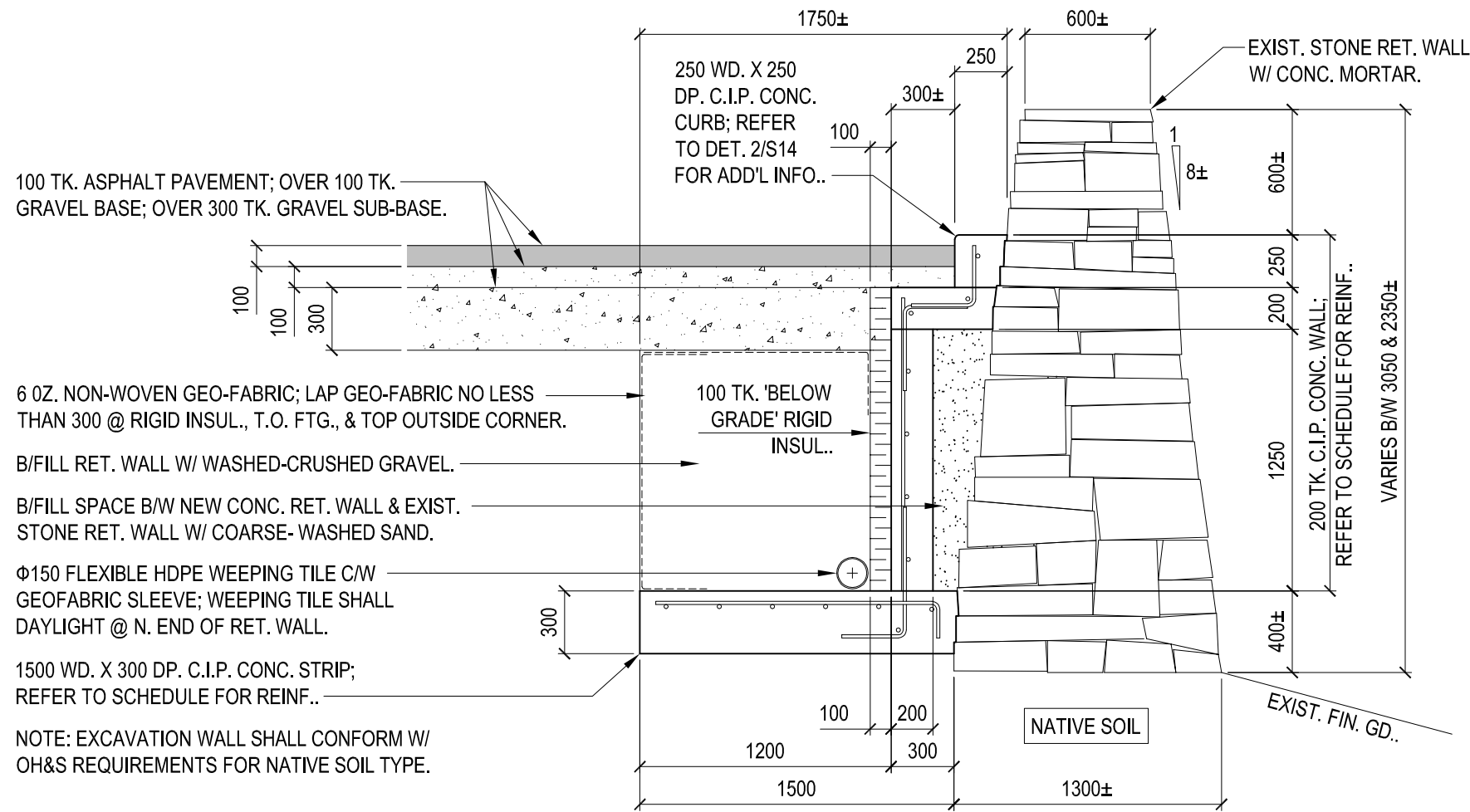
1 X-SECTION THRU. STONE RET. WALL. S11 SCALE - 1 : 30
