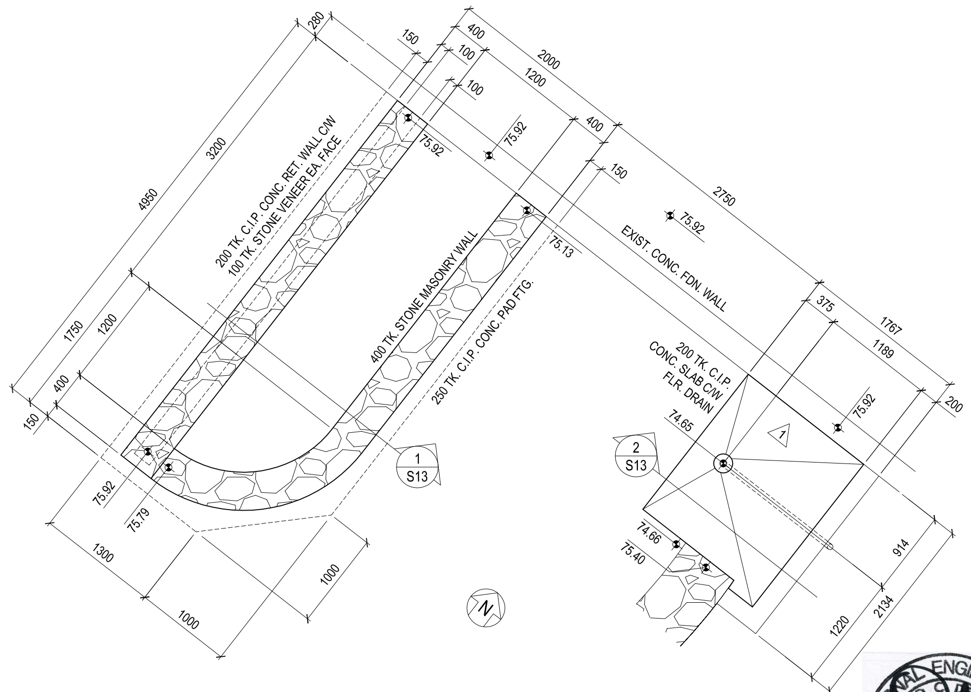
1 PARTIAL PLAN SHOWING NEW STONE WALL PLANTER & STORMWATER DRAIN. S12 SCALE - 1 : 40
