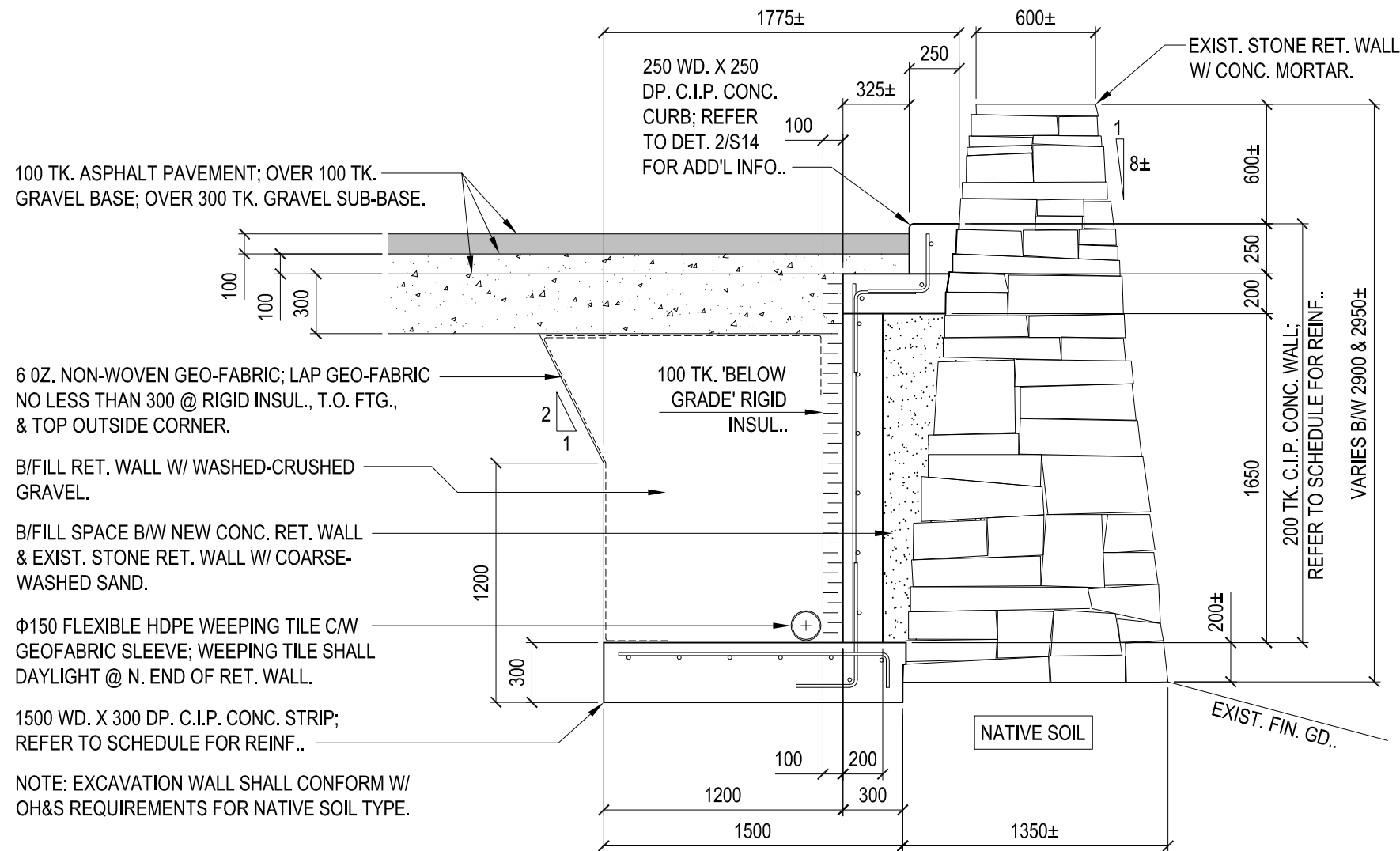
1 X-SECTION THRU. STONE RET. WALL. SCALE - 1 : 30
