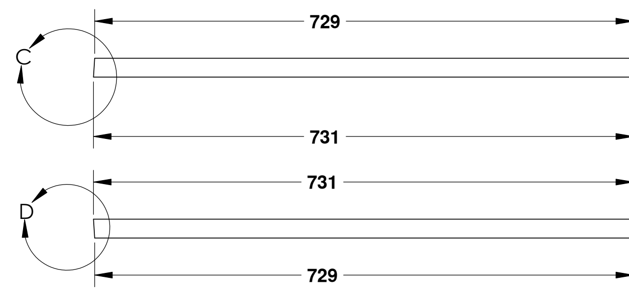
ROOF SUPPORT MATERIAL: ALUMINUM SQUARE TUBE 1 REQUIRED SCALE: 1:5
