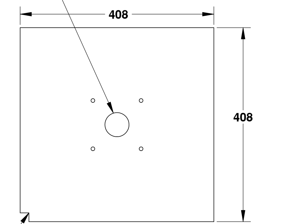
CAP PLATE MATERIAL: 10 GAUGE ALUMINUM 1 REQUIRED SCALE: 1:5
