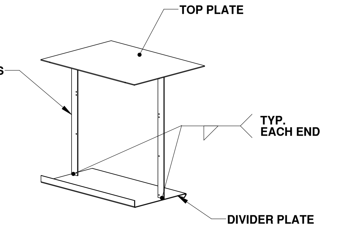
BREAKER PANEL ASSEMBLY LAYOUT
