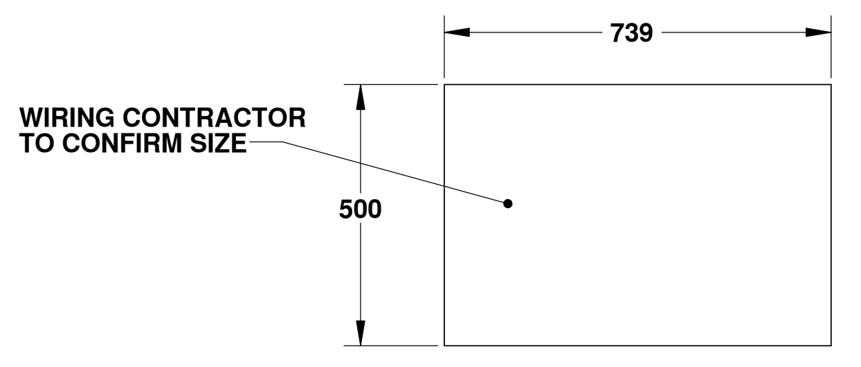
WIRING GUARD PLATE MATERIAL: 10 GAUGE ALUMINUM 1 REQUIRED SCALE: 1:10
