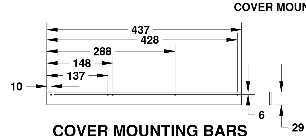
COVER MOUNTING BARS
