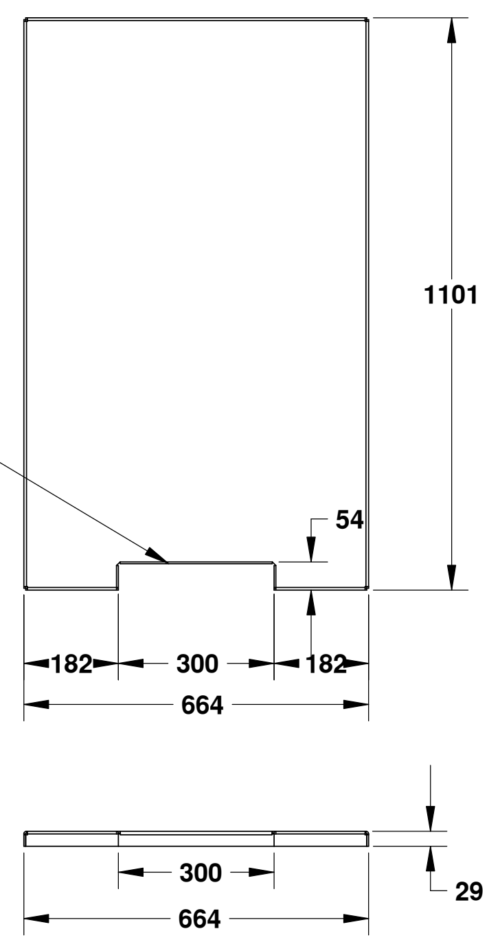
UPPER DOOR PANEL MATERIAL: 10 GAUGE ALUMINUM 1 REQUIRED SCALE: 1:10
