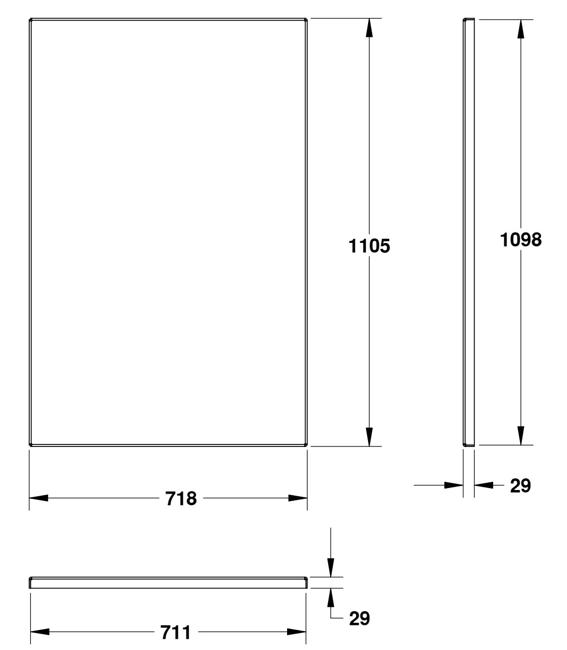
MAIN DOOR PANEL MATERIAL: 10 GAUGE ALUMINUM 1 REQUIRED SCALE: 1:10
