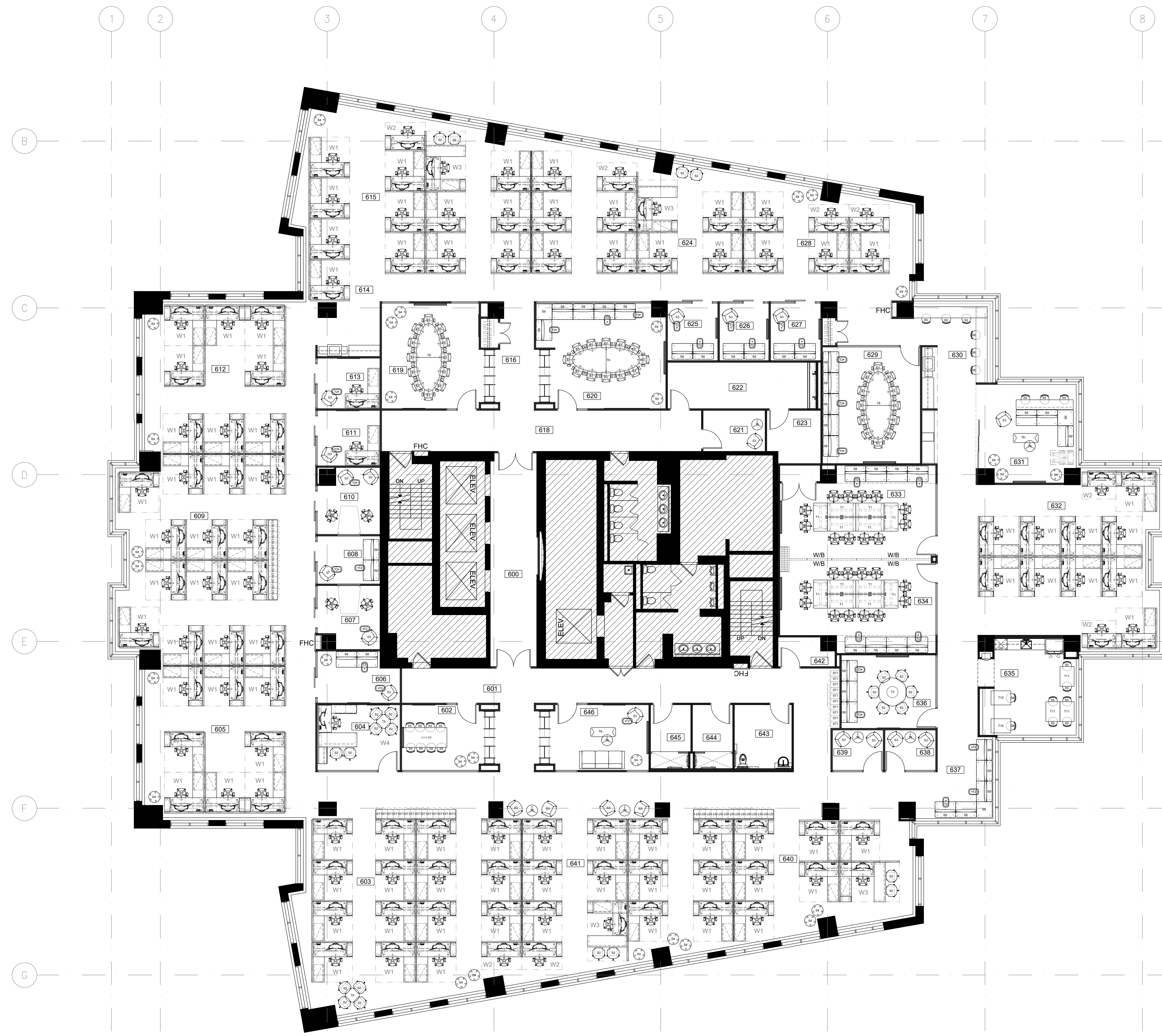
1 6th Floor Furniture Plan 4.0 | 4.0 Scale: 1:100
