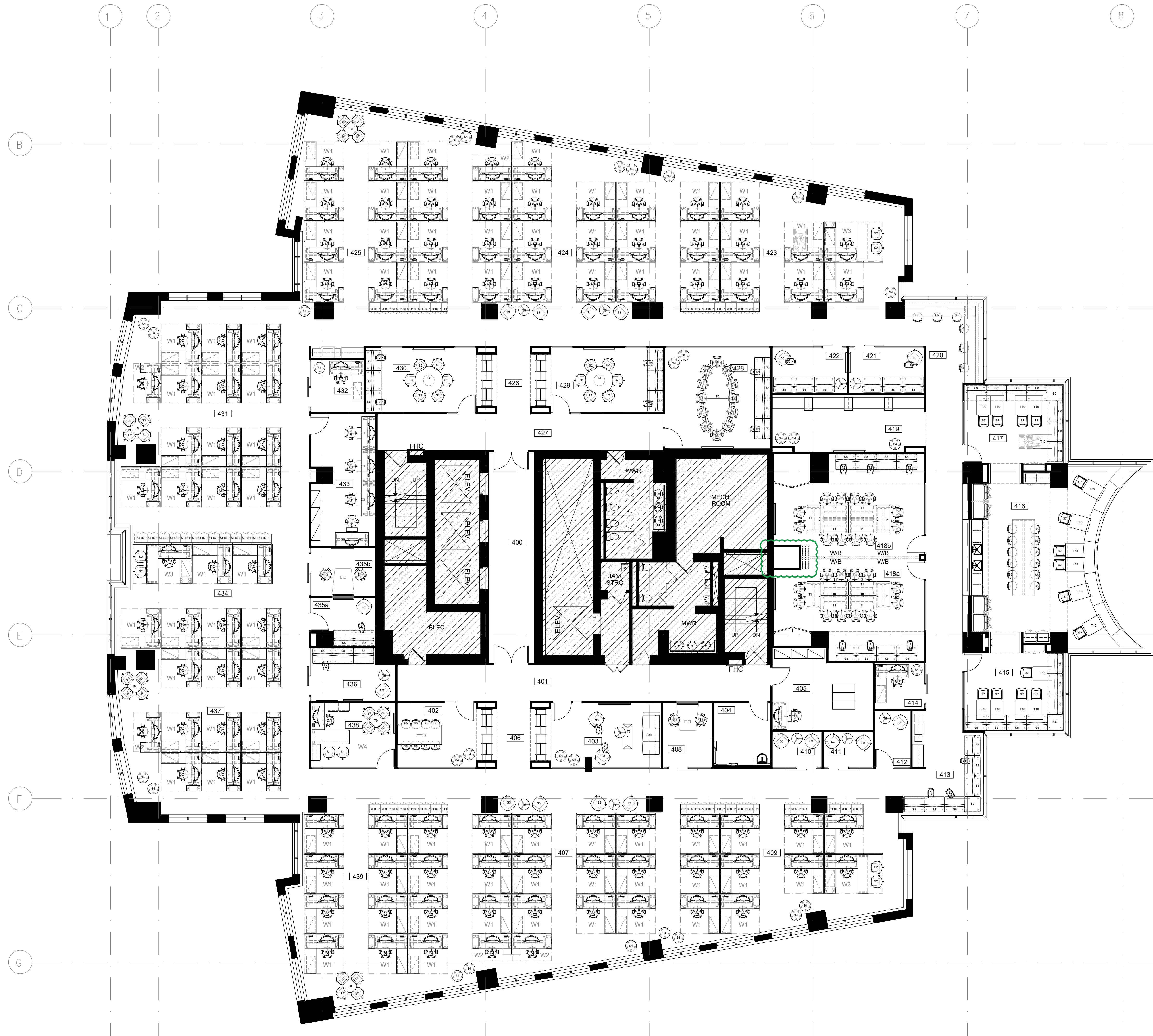
1 4th Floor Furniture Plan Scale: 1:100
