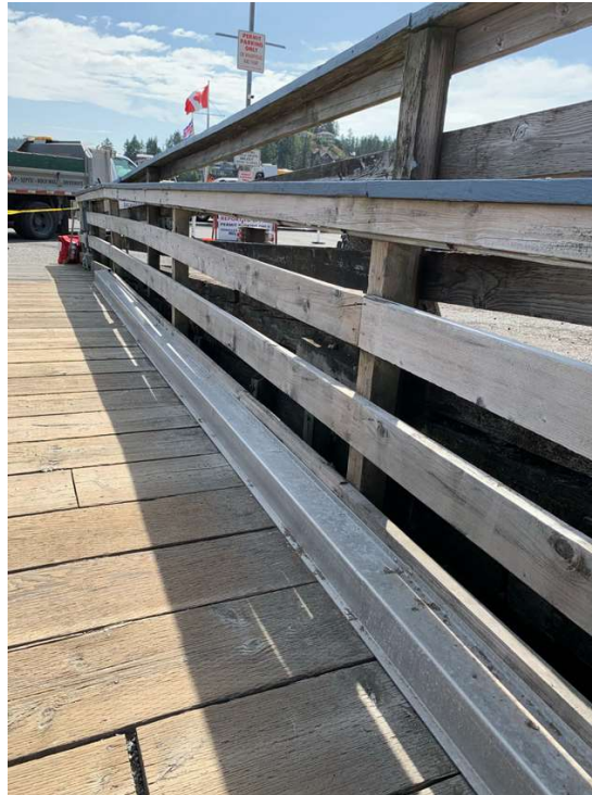
Potential Utility and Handrail Interference with Stringer Replacement
