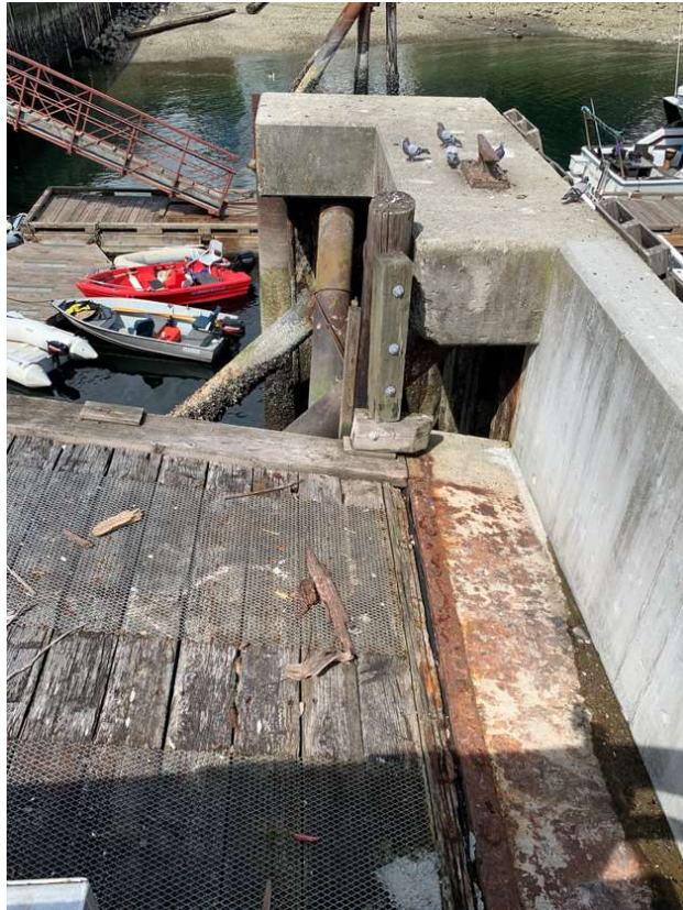
New Concrete Panels Installation Location (Old sloped ramp to be removed and new piles to be installed by others)
