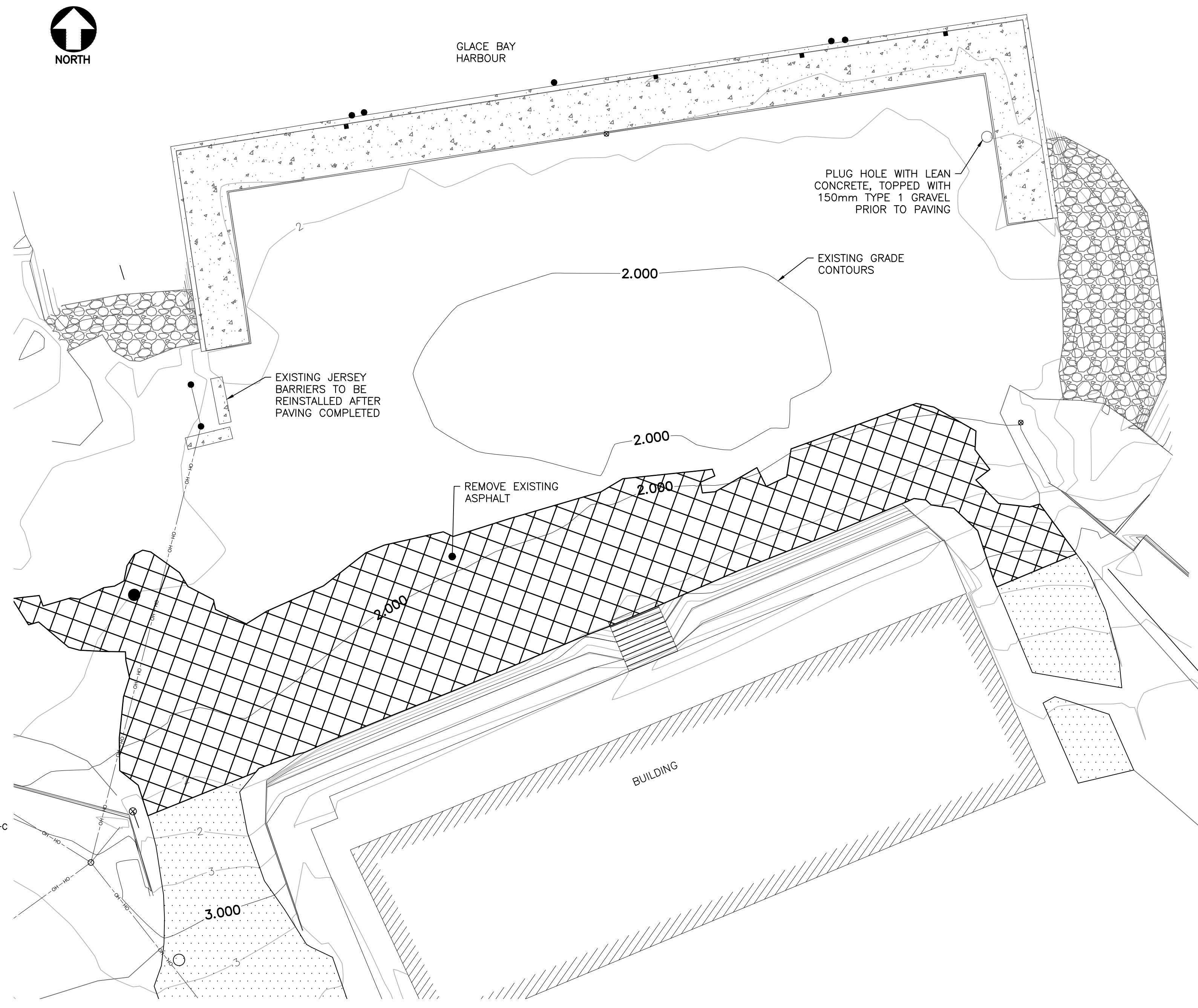
PLAN - REMOVALS SCALE : 1:150
