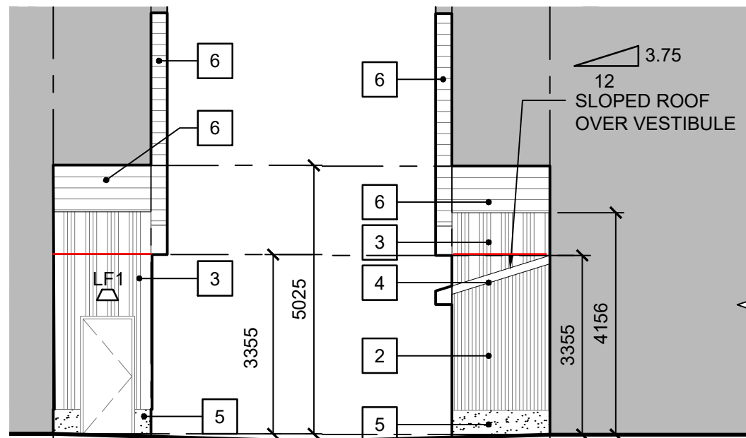
6 A-C-3.0 1:100 PARTIAL ELEVATION AT PARLOUR ENTRY
