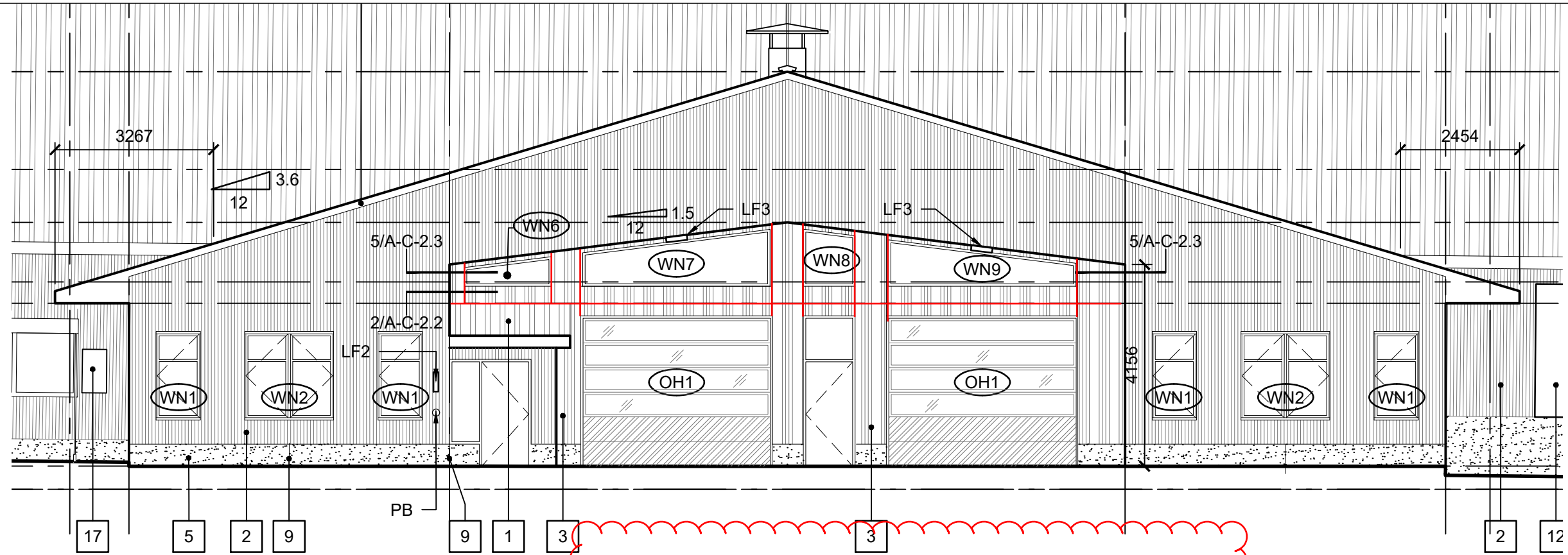
1 A-C-3.0 1:100 NORTH ELEVATION
