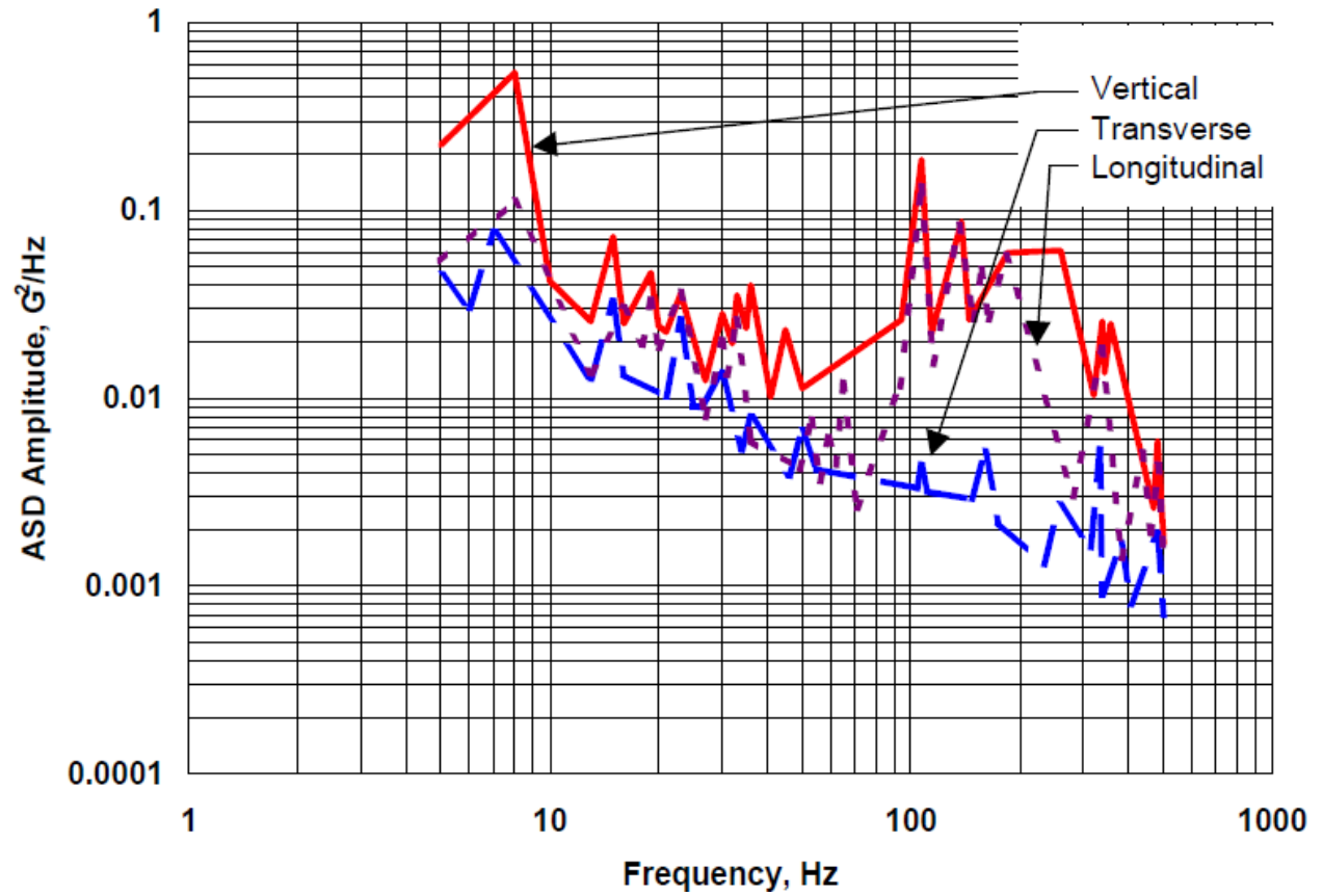
Figure A-3: Two-wheeled trailer
