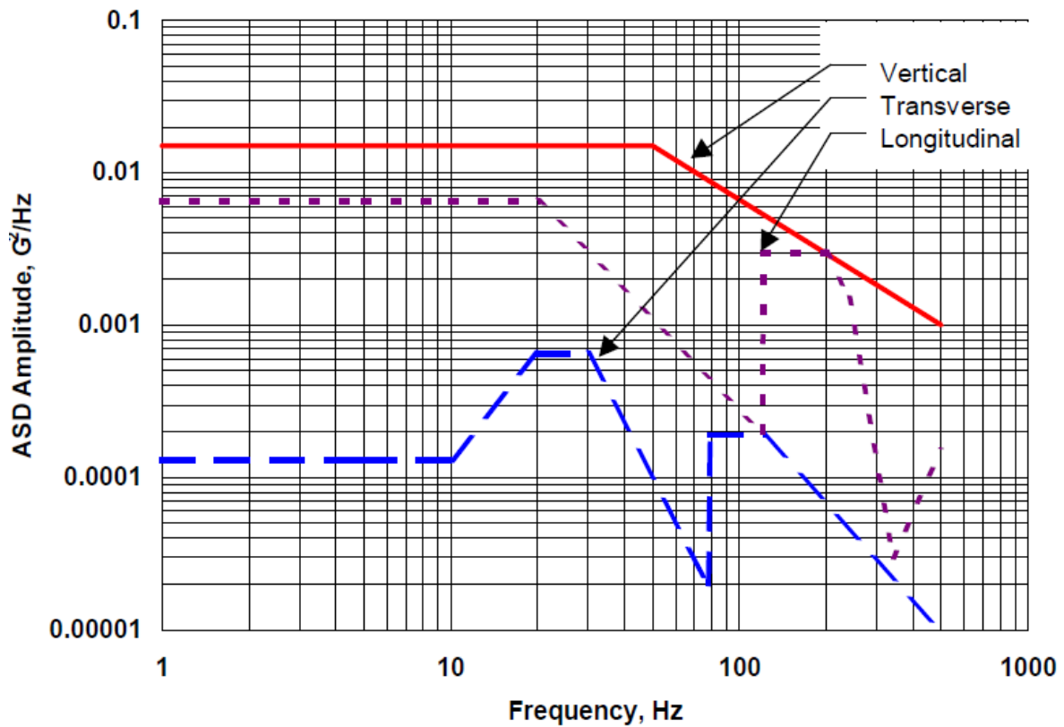
Figure A-1 : Ground Wheeled Common Carrier
