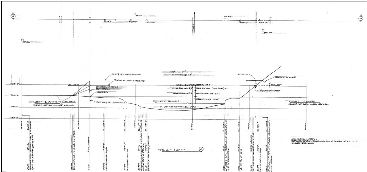
Figure 3: Chuchinka Creek Existing Structure
