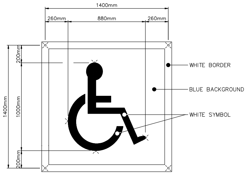
ACCESSIBLE PARKING SYMBOL NTS
