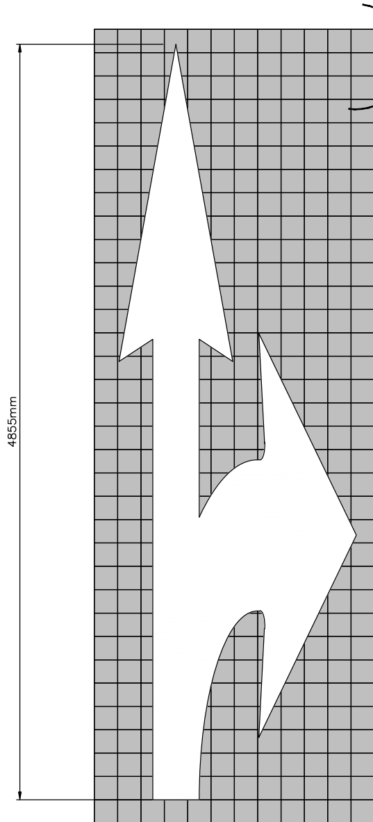
STRAIGHT THROUGH / RIGHT TURN NTS
