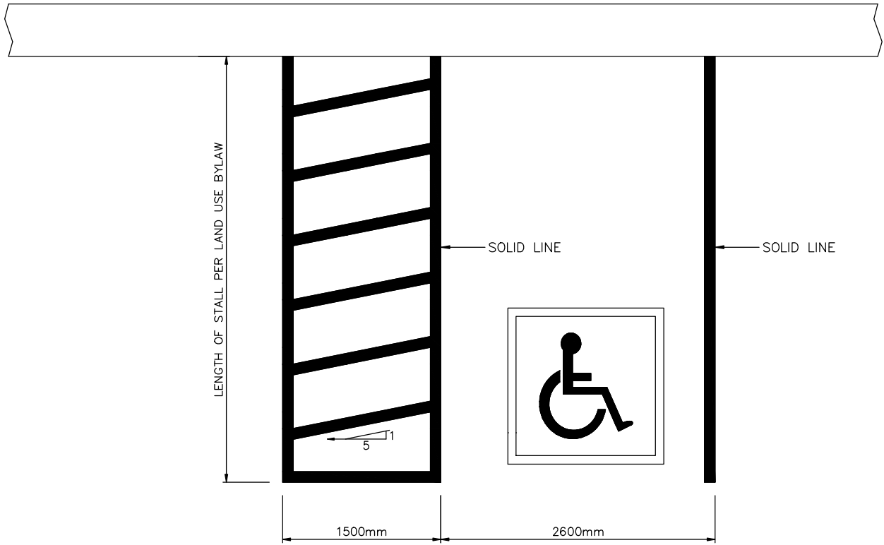
ACCESSIBLE PARKING STALL NTS
