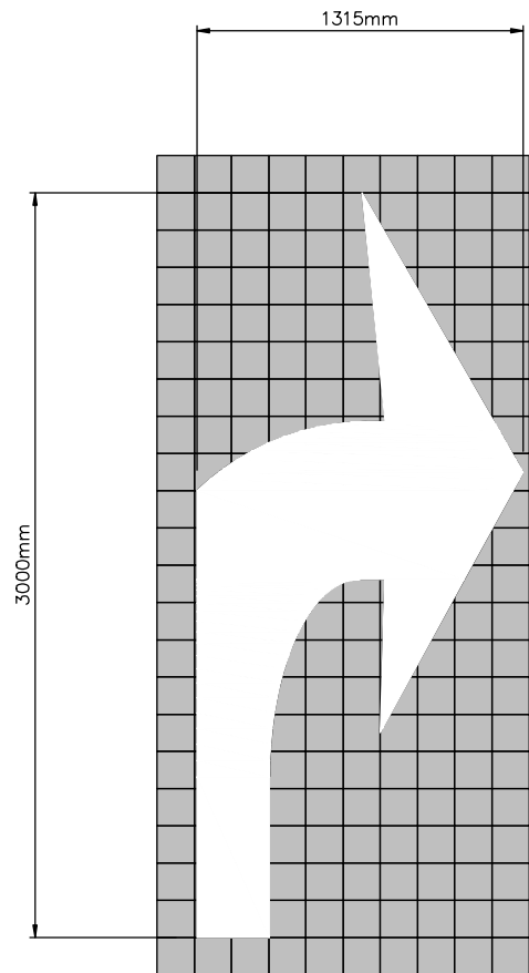
RIGHT TURN ONLY NTS
