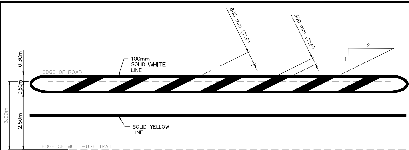
TYPICAL CHEVRON NTS
