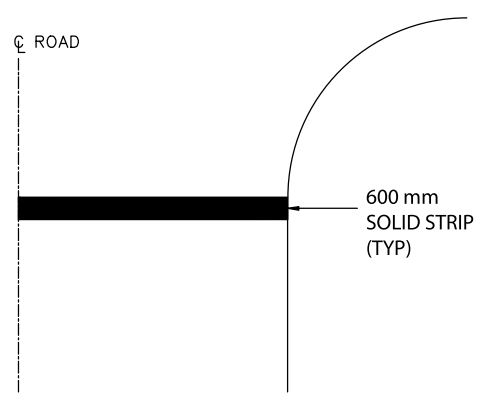
TYPICAL STOP LINE NTS
