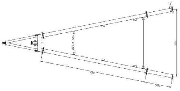
5. METRE A-FRAME EXACT HEIGHT TO CENTRE OF 25# WIRE ROPE IN MAIN CABLE SHEAVE = 5.24 METRES (WITHOUT FOOT PILES)
