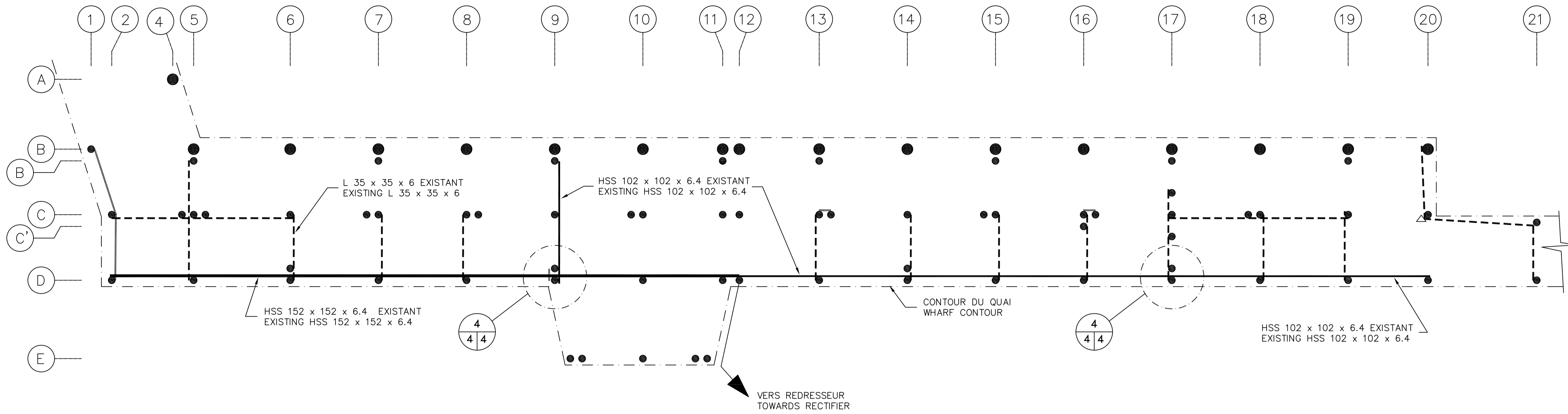
SCHEMA EN PLAN DE LA POSITION DES HSS ET DES CONTINUITES ELECTRIQUES PLAN DIAGRAM OF THE POSITION OF THE EXISTING HSS AND ELECTRICAL CONTINUITIES
