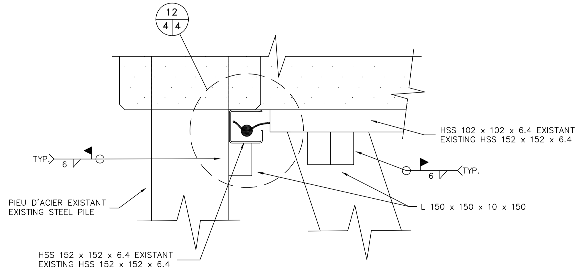
DETAIL TYPE – VUE VERTICALE TYPICAL DETAIL – VERTICAL VIEW
