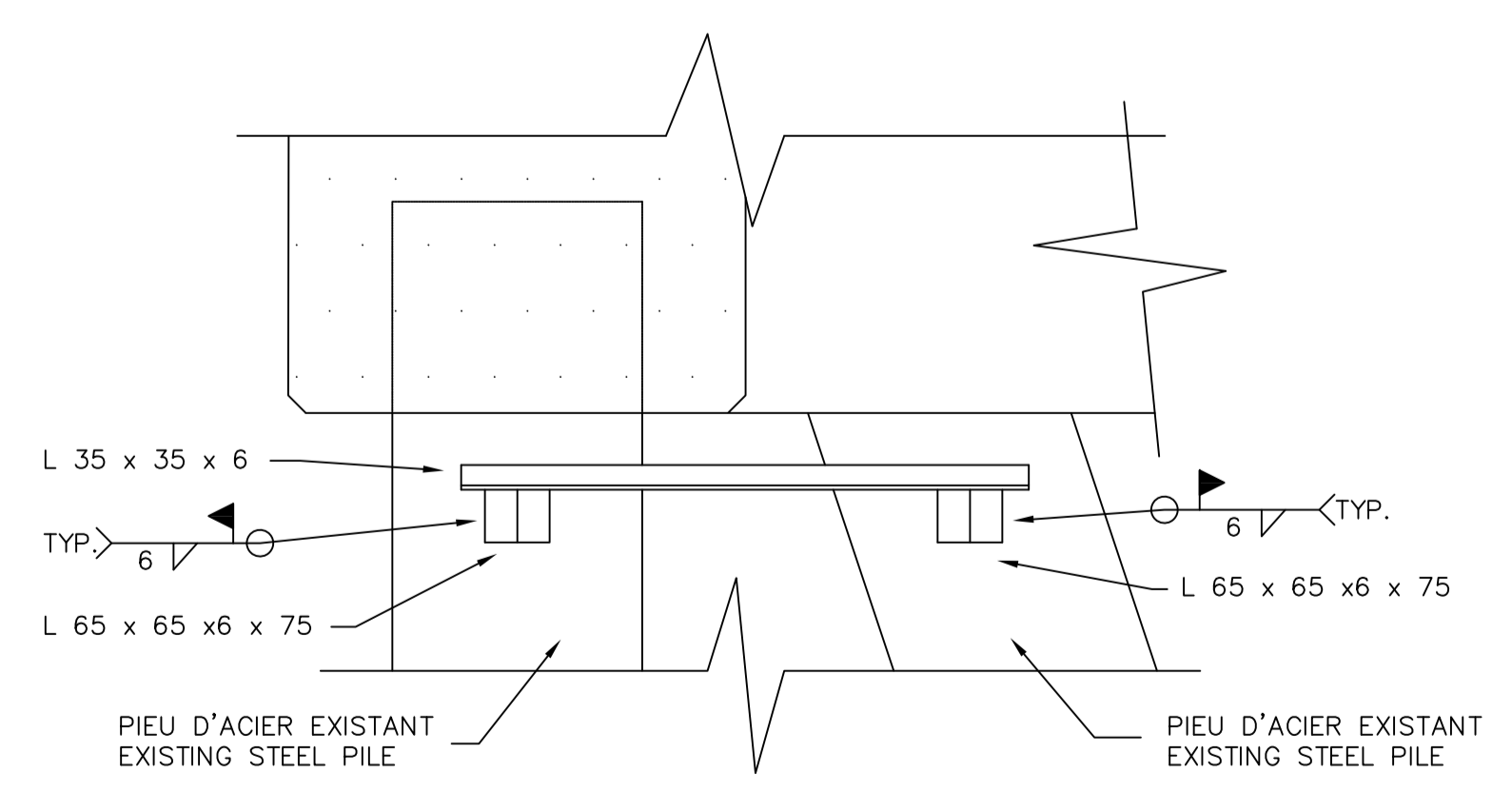
CONTINUITE ELECTRIQUE TYPE TYPICAL ELECTRICAL CONTINUITY
