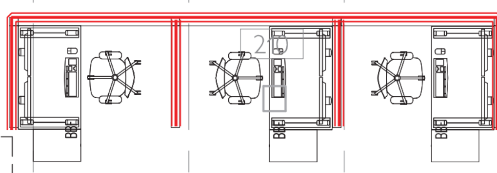
WORKSTATION PANELS - 3 DESKS IN MIDDLE OF ROOM (POWERED SPINE, FABRICTILES BACK TO BACK), DEMISING PANEL (FABRIC/FABRIC, NO POWER), 60"H X 60"W
