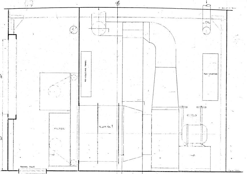
SECTION AT FRAMES 44 1/2 LOOKING FORWARD
