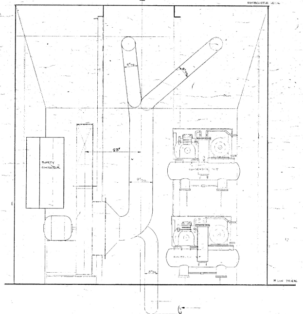
SECTION AT FRAMES 42 LOOKING AFT
