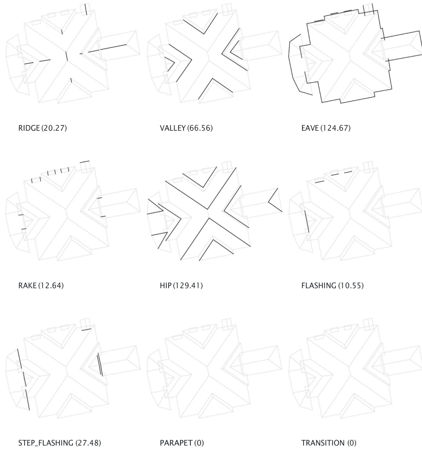
Figure 7: Roof Edge Classification (units: meters)
