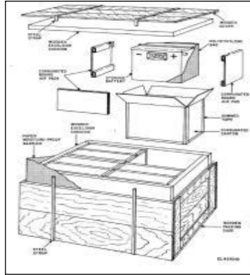
Fig 2. Example of a diagram of packaging
