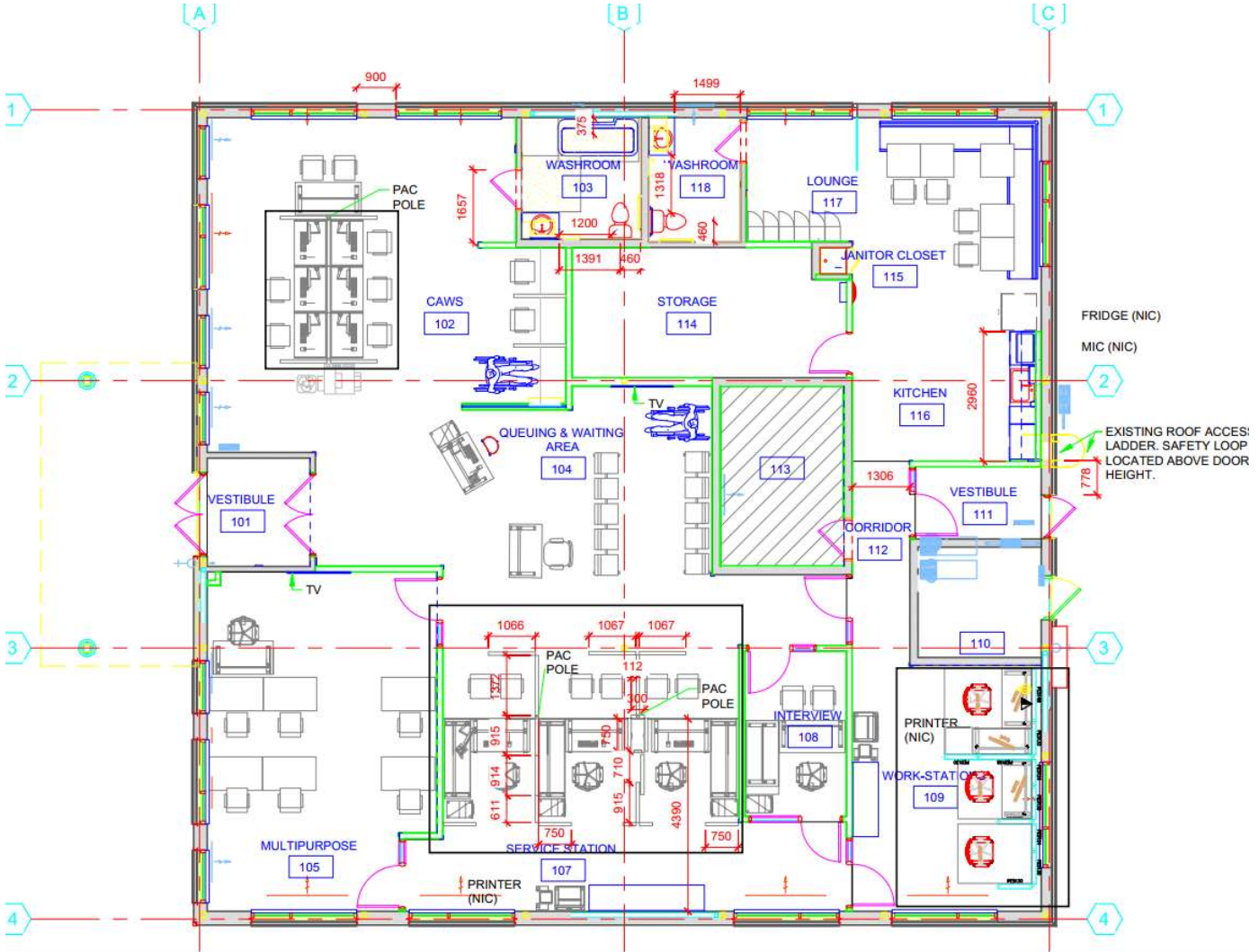
FLOORPLAN #1:
